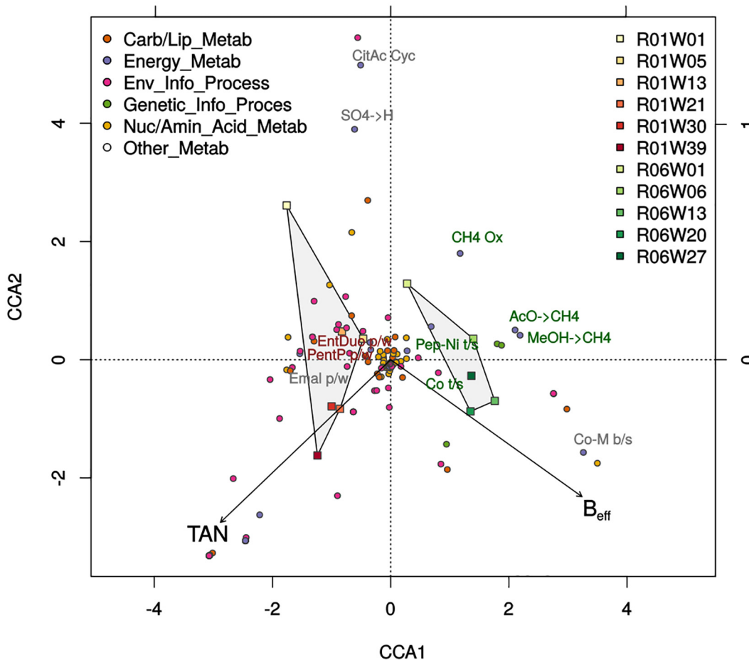
Fig 4. Ammonia levels (TAN) and biomethane conversion efficiency (B eff ) best differentiate predicted metabolisms between R1 and R6. Carbon metabolisms segregate along the X axis, reflecting divergent environments under the contrasting reactor setups. R1 samples ordinate more closely with diverse carbon metabolism (Entner-Doudoroff: EntDu p/w ; Pentose-Phosphate: PentP p/w ; ethymalonyl: Emal p/w ), while R6 samples ordinate strongly with methanogenic activities (Methanogenesis: AcO , MeOH → CH4 ; Co-Enzyme M biosynthesis: Co-M b/s ) and the uptake of trace elements (Cobalt: Co t/s ; Nickel: Pep-Ni t/s ). More diverse activities (Citric Acid Cycle: CitAc Cyc ; sulphate reduction: SO4->H ; methane oxidation: CH4 Ox ) ordinate closer to earlier samples, suggesting metabolic activities detrimental to biogas production were excluded as reactor communities developed. Activities in green represent strongest predicted biomarkers for R6, activities in red represent strongest predicted biomarkers for R1.
