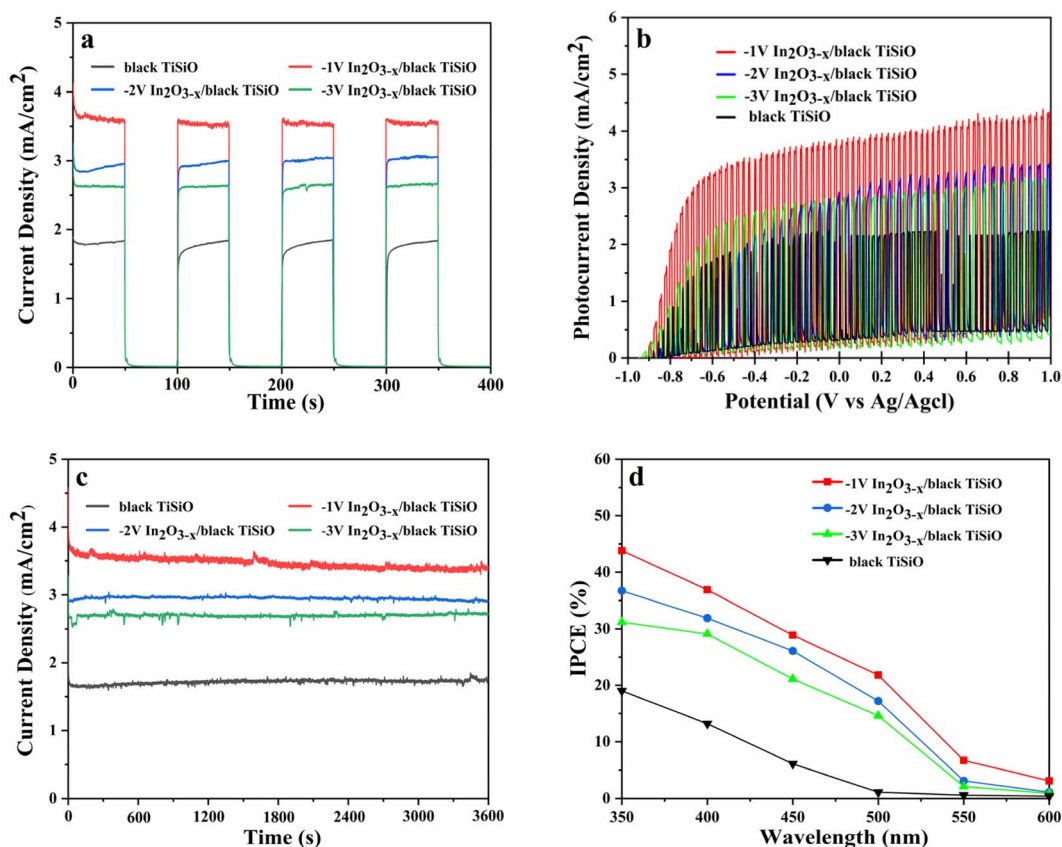
Fig. 7 (a) Transient I - t curves of the photoanodes at different deposition voltages, (b) transient linear sweep voltammetry (LSV) curves, (c) stability of photocurrent density for different composite photoanodes (0 V vs. Ag/AgCl), (d) IPCE of different photoanodes.
