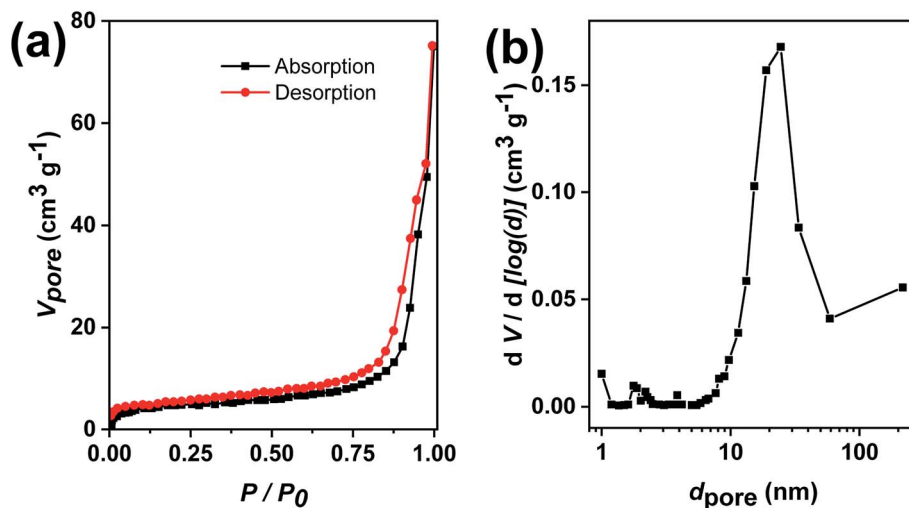
Fig. 7 (a) \text{N}_2 adsorption–desorption isotherms of Au@TiO 2 nanofibers and (b) corresponding pore size distributions of mesopores.
