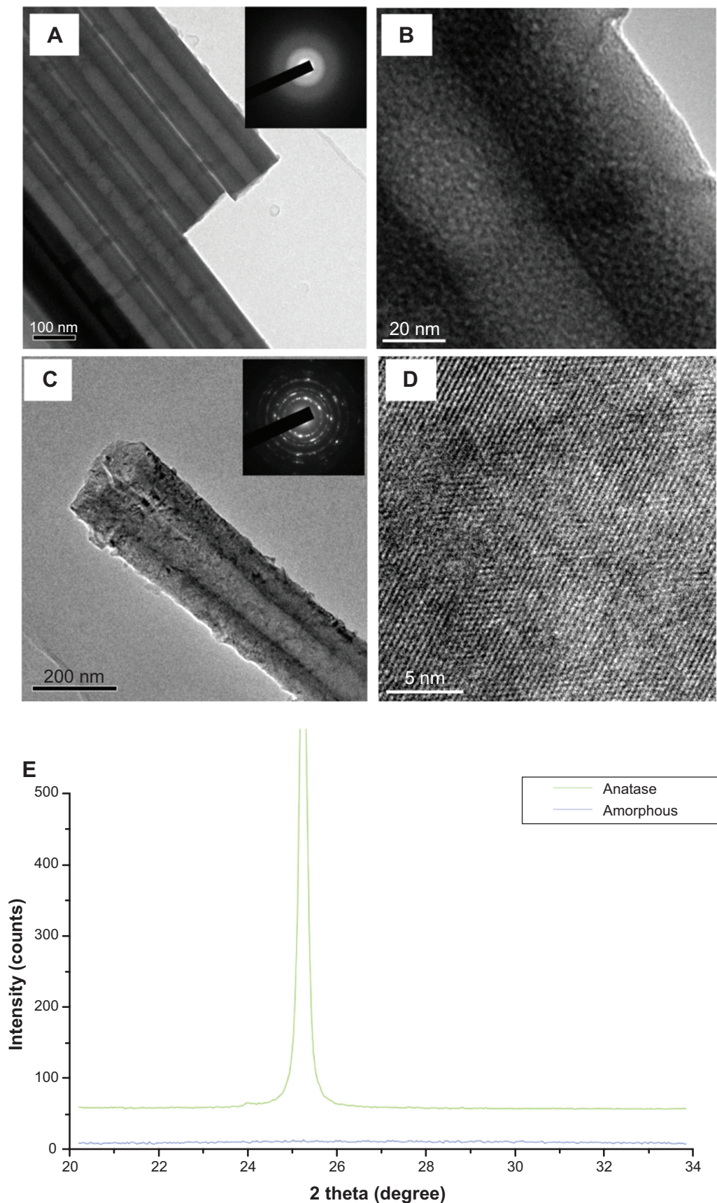
Figure 2 Transmission electron microscopy (TEM) images of (A–B) amorphous and (C–D) crystalline nanotubes are shown. (A and C) Show bright field TEM images of nanotubes. The insets are the corresponding diffraction patterns indicating (A) lack of crystallinity and (C) presence of crystalline structure. (B and D) Show high resolution TEM imaging that confirms atomic ordering at nanoscale. (E) X-ray diffraction data collected from amorphous and crystalline nanotubes. The crystalline nanotubes were identified as anatase phase.
