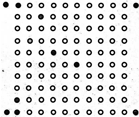
Figure 4 Tenplex reaction with complex genomic GMO DNA. 2.5% Bt176 maize and 2.5% RR soya in a tenplex with target DNA for seven padlock probes. Three padlock probes without target remain negative. For positioning of the spots, please consult Figure 3A.
