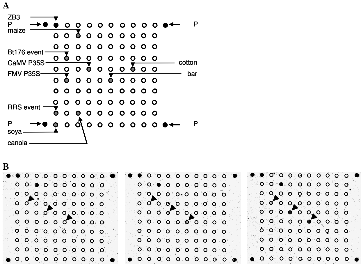
Figure 3 Microarray with the schematic position of the different padlock ZIP-codes (A) and hybridization results of a dilution series (0, 0.1 and 0.5%) of maize Bt176 (B). GMO maize was diluted in wild type maize. The expected hybridisation signal for maize (endogenous zein) is always present while CaMV P35S and bar (in 0.1%) and Bt176 event (0.5%) emerge when the concentration increases. Arrows indicate the appearance of the Bt176 event, CaMV P35S and bar spots.
