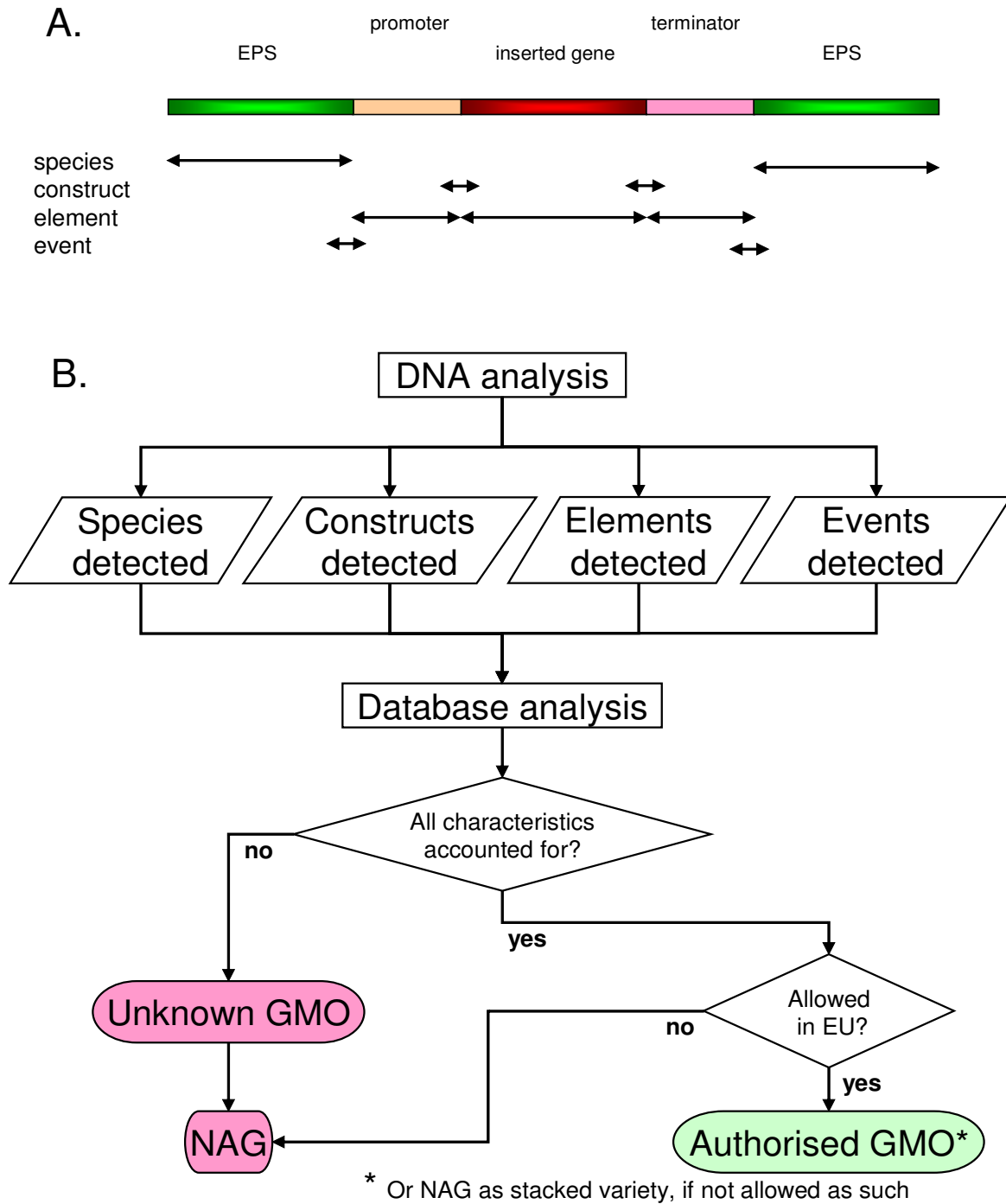
Figure 1 Padlock probe locations in a GMO and GMO decision tree. Scheme for the location of specific padlock probes on species-, construct-, element- and event level of a GMO. EPS = endogenous plant sequence (A). GMO decision tree in which the outcomes of DNA analyses are matched with the data from a database on known GM crop events to elucidate the presence and status of GMOs in a test sample. Here, events, elements, constructs and species are detected and compared with the database information. Detection of unknown GMOs is by exclusion of profiles of known GMOs present within the sample (B).
