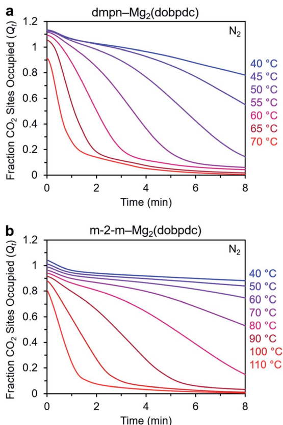
Fig. 11 Desorption of \text{CO}_2 under dry \text{N}_2 from (a) dmpn- \text{Mg}_2(\text{dobpdc}) and (b) m-2-m- \text{Mg}_2(\text{dobpdc}) . In each experiment, the sample was allowed to equilibrate under pure \text{CO}_2 at the indicated temperature, after which the gas stream was switched to \text{N}_2 . In these plots, data are normalized such that t = 0 corresponds to the data point immediately before mass decrease was observed due to \text{CO}_2 desorption (i.e., t = 0 is after the 19 s delay prior to \text{N}_2 reaching the sample in the furnace).
