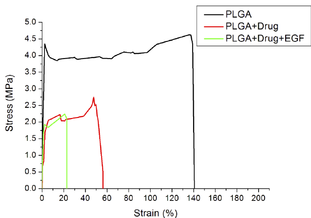
Figure 6 Stress-strain curve of pure PLGA, lidocaine-incorporated, and lidocaine/hEGF-loaded sheath-core-structured nanofibers. Abbreviations: hEGF, human epidermal growth factor; PLGA, poly[(d,l)-lactide-co-glycolide].
