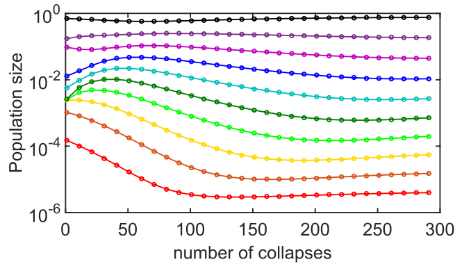
Figure 3. Transient dynamics in Kill-the-King model with N=10 species that grow equally fast and collapse to a fixed population \gamma = 10^{-6} . For clarity we show the state of the model only every 10 collapses, that is to say, after each species collapsed exactly once so that the population order is maintained. The steady state of KtK model where all ratios \delta_i between rank-ordered populations are equal to each other and to \gamma^{1/N} is approximately reached already after 300 collapses. The relaxation to this steady state is described by the discrete anisotropic Burgers equation 5 or its continuous counterpart Eq. 6.
