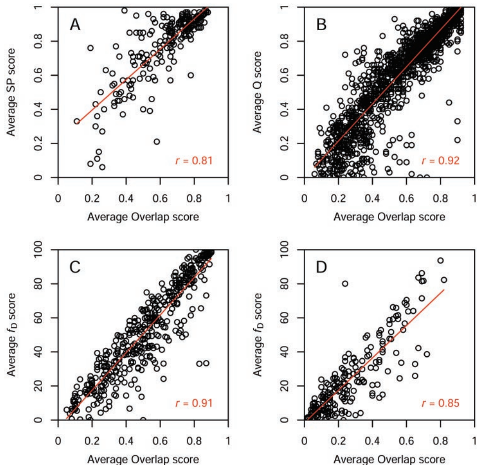
Figure 2. Scatter-plots of estimated case difficulty using the average overlap score versus real difficulty: Balibase (A), Prefab (B), SABmark superfamily (C) and SABmark twilight (D). The Pearson correlation coefficient ( r ) is high for all test sets.
