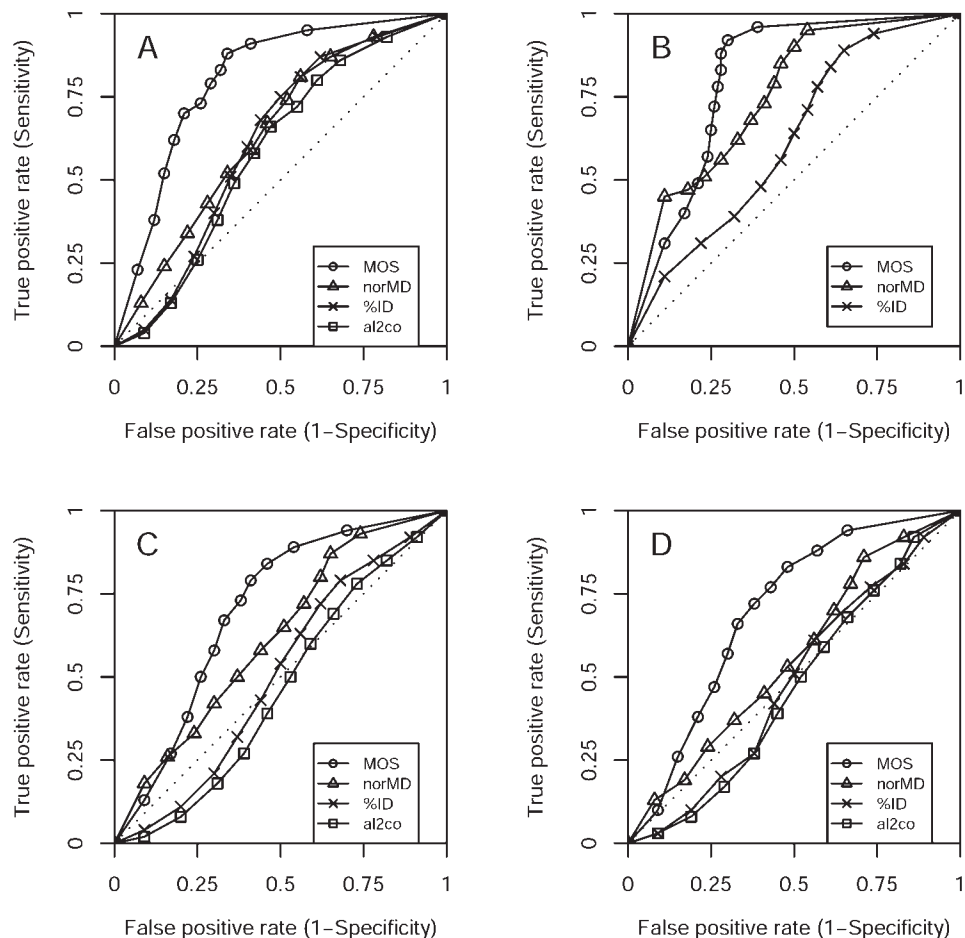
Figure 3. ROC curves demonstrating the agreement between real and predicted rank of several alignments of the same sequences: Balibase (A), Prefab (B), SABmark superfamily (C) and SABmark twilight (D). For al2co, we only show the best curve among all 9 combination of methods (Table 3, italic). For the Prefab set no meaningful results could be obtained using al2co. The rankings based on our MOSs are more accurate than the rankings according to norMD, al2co and sequence identity scores, accepting fewer false positives at comparable levels of true positives. The predictions of all scores are less accurate on the SABmark sets than on Balibase and Prefab.
