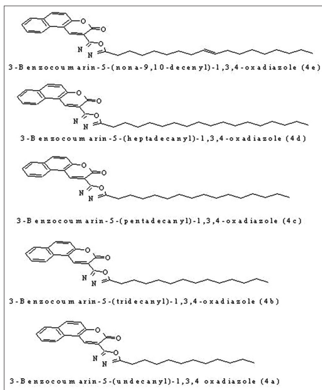
Fig. 1: Structures of 2-(5-alkyl-1,3,4-oxadiazol-2-yl)-3H-benzo[ f ]chromen-3-ones (4a-e)
