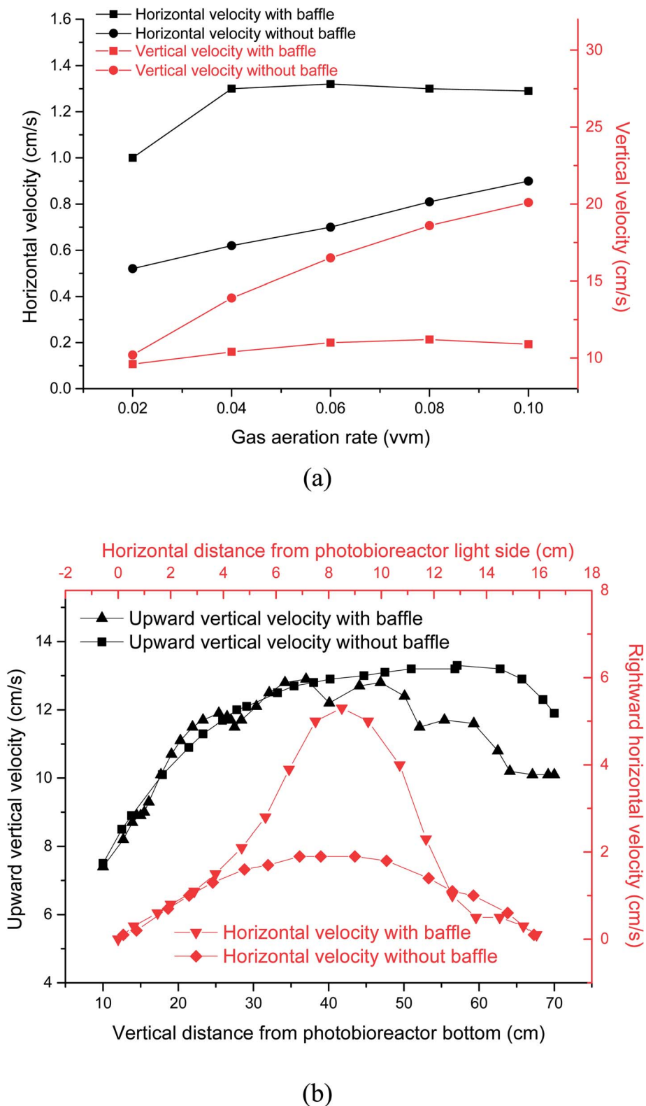
Fig. 3 Vertical velocity and horizontal velocity of fluid in a panel bioreactor with horizontal baffles. (a) Vertical velocity and horizontal velocity under different gas aeration rate (b) vertical velocity and horizontal velocity at different position in a panel bioreactor under gas aeration rate of 0.02 vvm.
