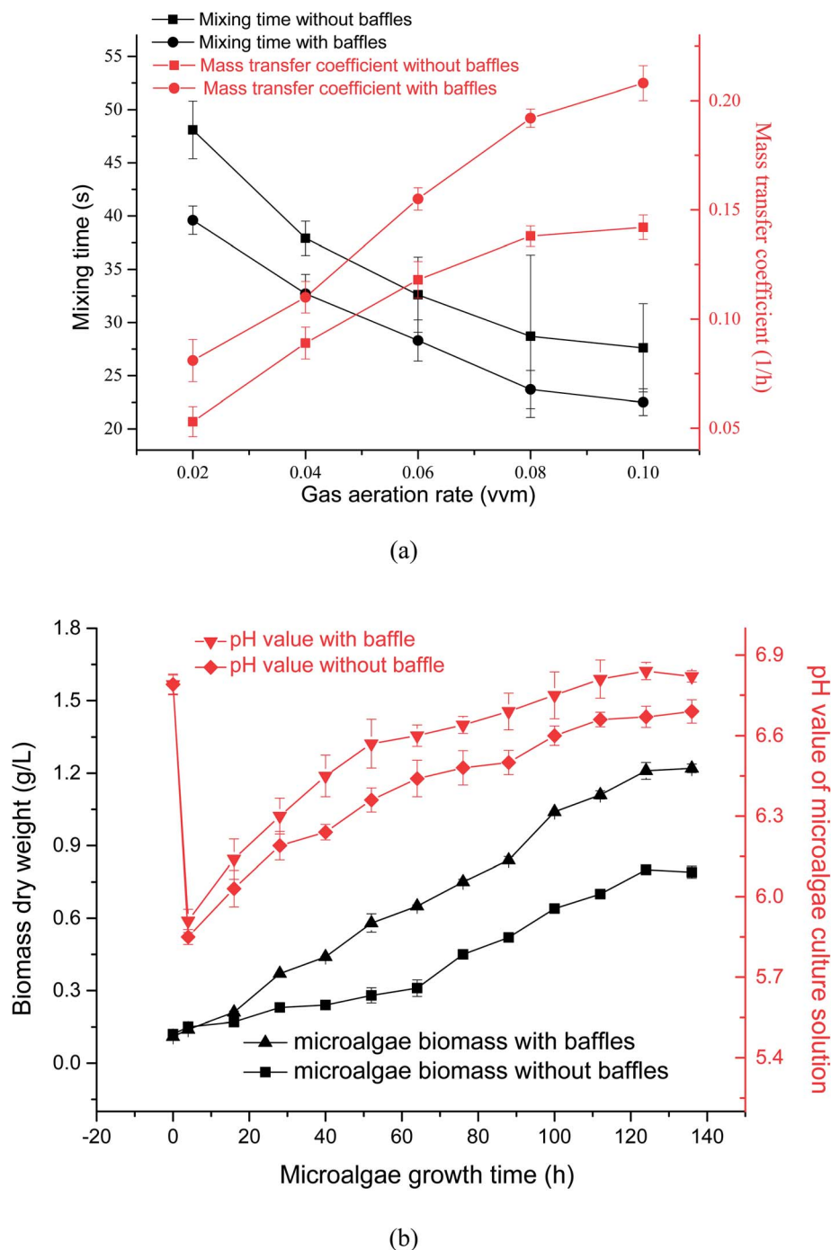
Fig. 6 Microalgal growth in an optimized flow field of a panel bioreactor with horizontal baffles. (a) Effects of gas aeration rate on mixing time and mass transfer; (b) effects of horizontal baffles on pH and microalgal growth.
