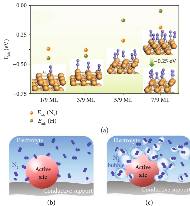
FIGURE 1: Computational studies and schematics of the conventional and adjusted reaction interface. (a) DFT calculations on the effect of \theta_{N_2} on E_{\text{ads}}(\text{H}) on the Pd(100) surface. White and purple balls denote H and N, respectively. (b) Schematic of the traditional solid-solution two-phase interface. (c) Schematic of the adjusted gas-solid-solution three-phase interface.
