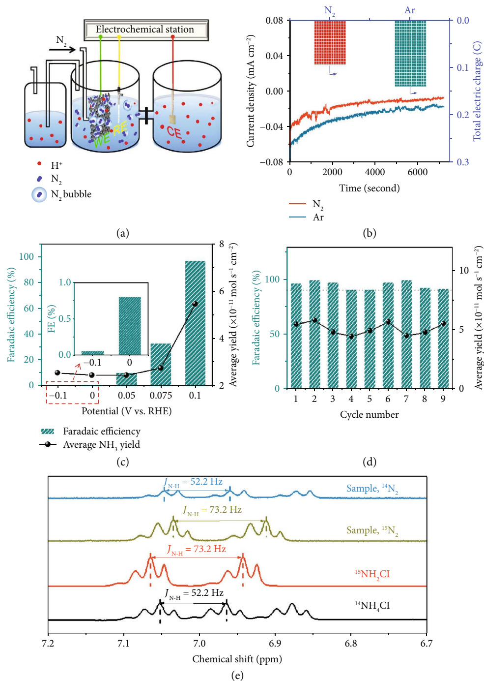
FIGURE 3: Electrochemical NRR performances of the Pd/ACC catalyst. (a) Schematic of the NRR device. (b) Chronoamperometry curve and total electric charge after electrolysis of Pd/ACC in \text{N}_2 or Ar at 0.1 V for 2 h. (c) FE and average yield rate of \text{NH}_3 production at various potentials based on the indophenol blue method with an inset of an enlarged figure. (d) Nine times recycling NRR experiments of a Pd/ACC electrode tested at 0.1 V for 2 h. (e) Isotope labelling experiment. 600 \text{ M } ^1\text{H} NMR spectra were obtained after electrolysis in 0.1 M HCl with ^{15}\text{N}_2 and ^{14}\text{N}_2 as the feeding gas. The multiplet splitting of the peaks may be because of the deuterated derivatives of ammonium.
