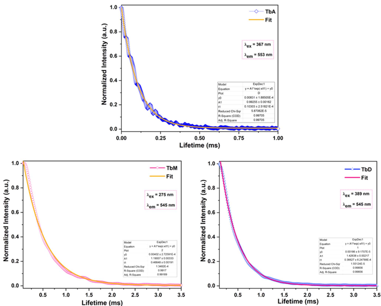
Fig. 8 Decay time-profiles of TbA–TbD.
