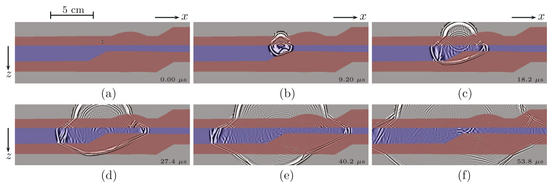
Figure 3. Virtual response G(r, s, t) + G(r, s, -t) , retrieved from the single-sided ultrasonic reflection response G(x', x, t) of the physical model in Fig. 2(a). (a) t = 0 \mu\text{s} . (b) t = 9.2 \mu\text{s} . (c) t = 18.2 \mu\text{s} . (d) t = 27.4 \mu\text{s} . (e) t = 40.2 \mu\text{s} . (f) t = 53.8 \mu\text{s} .
