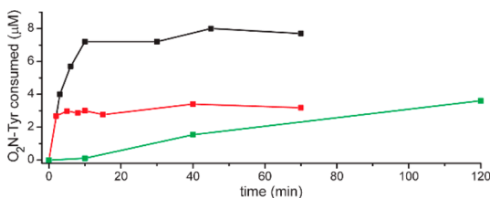
Figure 3. Reduction of O 2 N-Tyr by enzyme-bound and free FMN hq . Consumption of O 2 N-Tyr (8 μM) by alternative addition of the reduced form (18 μM) of wt hhIYD (red points and line), its T173A mutant IYD (black points and line), and free FMN hq (green points and line) under anaerobic conditions was monitored over time by reverse-phase HPLC (see Figure S3).
