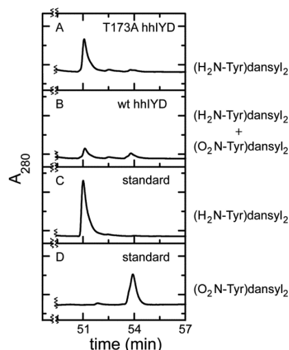
Figure 4. Detection of the O 2 N-Tyr reduction product after derivatization by dansyl chloride. O 2 N-Tyr (8 μM) was alternatively treated under anaerobic conditions for 50 min with (A) the reduced mutant T173A (18 μM) and (B) the reduced wt hhIYD (18 μM). (C) A standard of H 2 N-Tyr. (D) A standard of O 2 N-Tyr. Each sample and standard was ultimately treated with dansyl chloride (500 μM) before separation on reverse-phase C-18 HPLC using a gradient of solvent A (25 mM ammonium formate pH 5.7 and 14% acetonitrile) and B (acetonitrile) according to 0% B for 0–5 min; 0–8% B from 5 to 10 min; 8% B from 10 to 25 min; 8–45% B from 25 to 55 min; 45–58% B from 55 to 60 min (1 mL/min).
