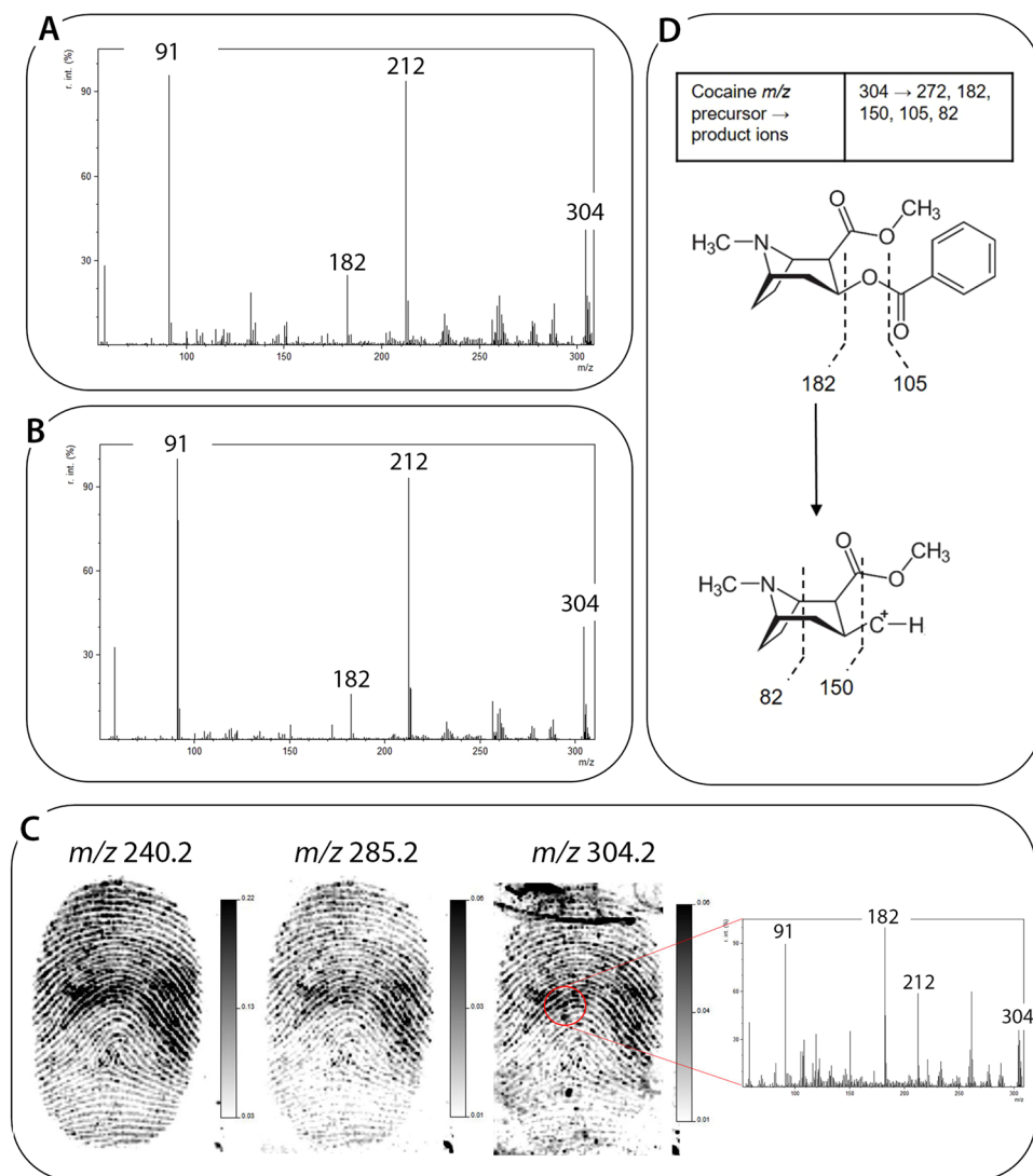
Figure 7. (A) MALDI MS/MS confirmation of 10 ng/mL cocaine spotted onto a polymer banknote, (B) MALDI MS/MS confirmation of 100 ng/mL cocaine spotted onto a latent ungroomed fingerprint deposited onto a polymer banknote, (C) MALDI MS images of an unidentified species and protonated stearic acid ( m/z 240.2 and m/z 285.2, respectively) and cocaine ( m/z 304.2) of a fingerprint contaminated with 100 \mu L of 100 ng/mL cocaine (10 ng total drug), followed by post-image MALDI MS/MS confirmation of cocaine and (D) the accepted fragmentation pattern of cocaine.
