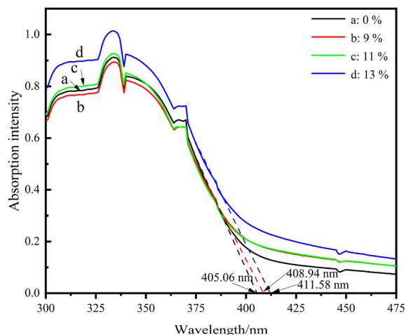
Fig. 5 UV-Vis-Abs of various LDHs/LM-TiO 2 .
