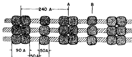
TEXT-FIG. 3. Model devised to account for the observed cross-striations in fully polymerized fibrin as shown in Fig. 4.
