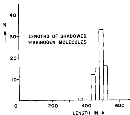
TEXT-FIG. 1. Histogram showing distribution of measured lengths of shadowed fibrinogen molecules.
