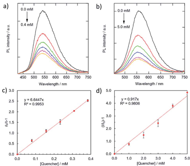
Fig. 6 Variations in PL spectra (a, b) and the corresponding Stern-Volmer-type plots of the quenching (c, d) for the combinations of the g-CDs with Cu 2+ (a, c) and the y-CDs with Fe 3+ (b, d).
