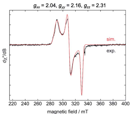
Fig. 7 Molecular structure of trans -[Ni I (Mes 2 Im) 2 (C 6 F 5 ) 2 ] ( 11 ) (top) in the solid state (ellipsoids drawn at the 50% probability level) and EPR spectrum at –203 °C of the isolated compound 11 (bottom). Hydrogen atoms are omitted for clarity.
