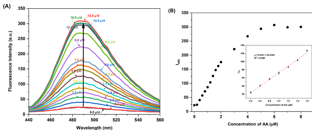
Fig. 4 (A) Fluorescence titration spectra of ProN6 (2 \mu\text{M} ) after mixing with various concentrations of AA (0–16 \mu\text{M} ) in ethanol. The excitation wavelength was 300 nm; (B) the plot of fluorescence intensity of ProN6 at 490 nm against varied concentrations of AA. Inset: selected range of a linear relationship between the concentration of AA ( \mu\text{M} ) and the fluorescence intensity at 490 nm ( I_{490} ).
