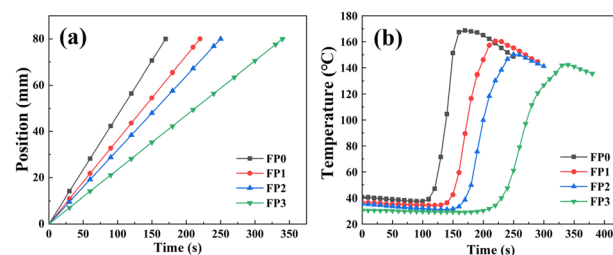
Fig. 3 (a) Speed of hydrogel polymerization frontal; (b) temperature of hydrogel polymerization frontal.
