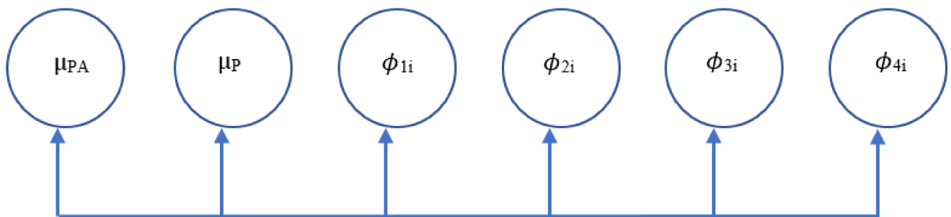
Figure 3. VAR(1) Model: Between-Person. Note. Figure 3 depicts the between-person components of the study model. PA represents physical activity, P represents pain, \mu represents between-person means, and \phi represents autoregressive parameters.
