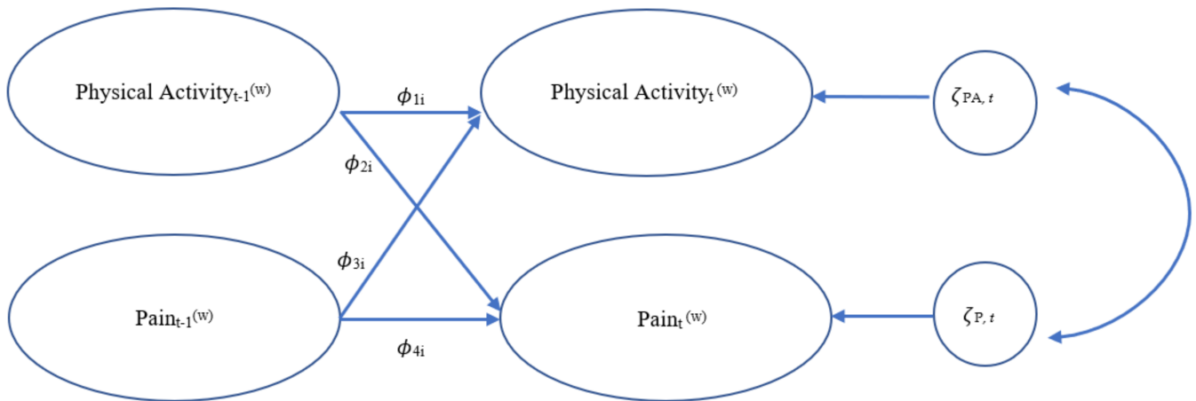
Figure 2. VAR(1) Model: Within-Person. Note. Figure 2 depicts the within-person components of the study model. T represents time point, t–1 represents previous time point, \phi represents autoregressive parameters (how quickly an individual restores to equilibrium) and cross-lagged regression effect (predictive relationships/spill-over), PA represents physical activity, P represents pain, and \zeta represents dynamic errors.
