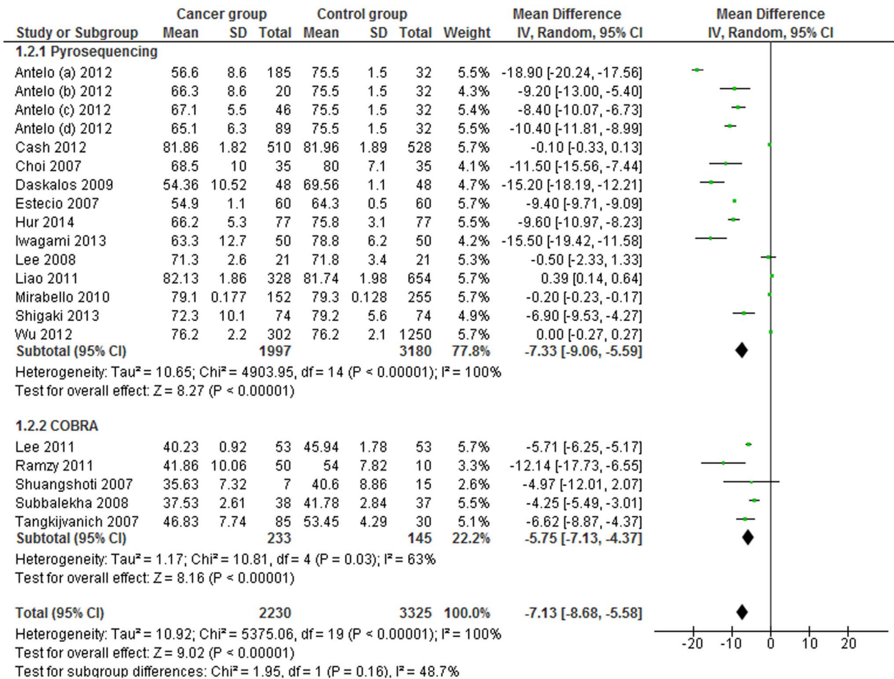
Figure 5. Forest plot of the mean difference of LINE-1 methylation levels between cancer and control groups. Subgroups analysis based on method. doi:10.1371/journal.pone.0109478.g005
