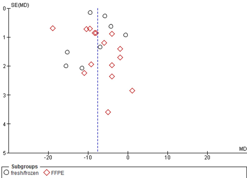
Figure 8. Funnel plot. Subgroup analysis based on tissue specimen types. SE, standard error, MD, mean difference. doi:10.1371/journal.pone.0109478.g008
