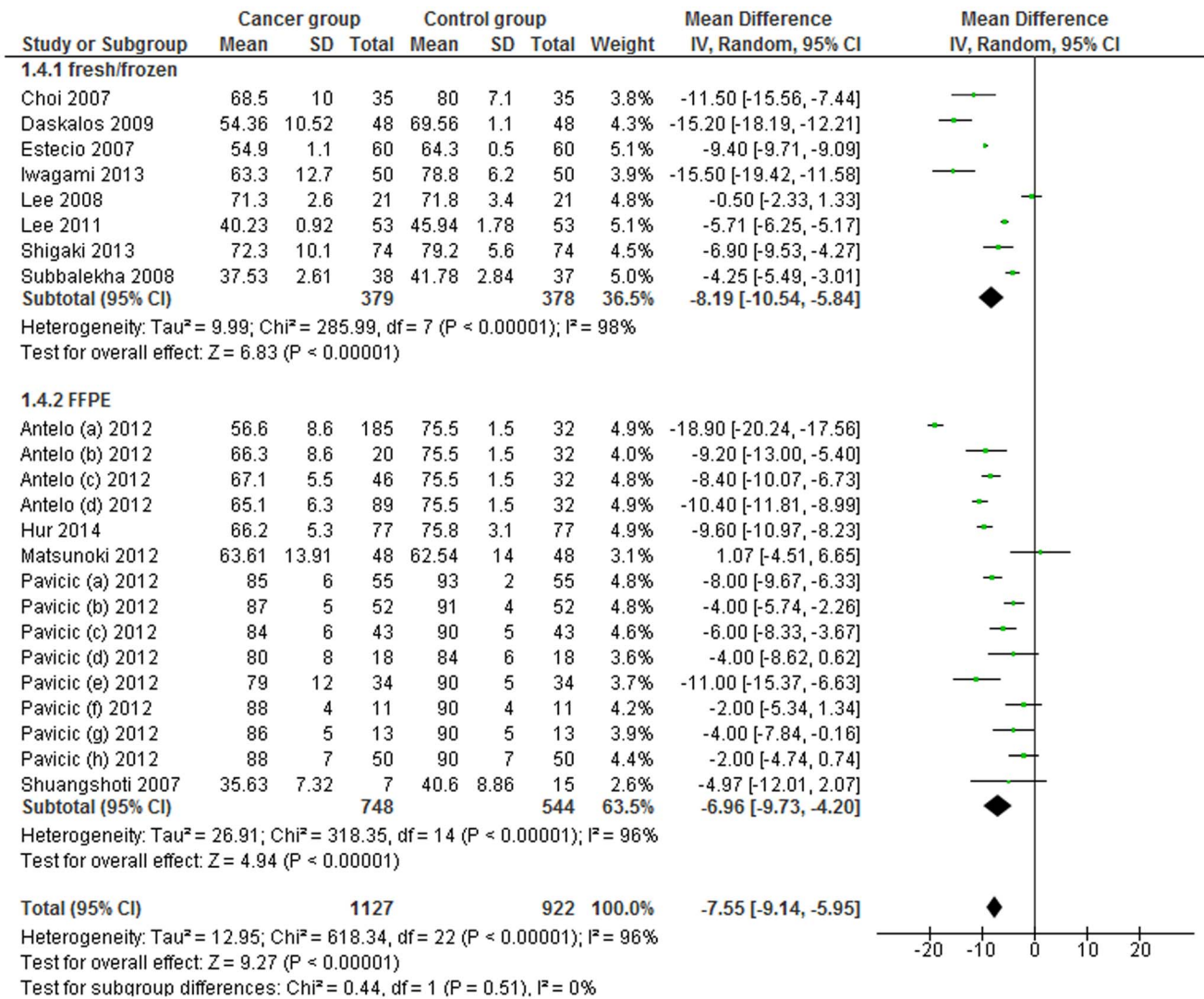
Figure 3. Forest plot of the mean difference of LINE-1 methylation levels between cancer and control groups in tissue samples. Subgroups analysis based on sample source. doi:10.1371/journal.pone.0109478.g003
