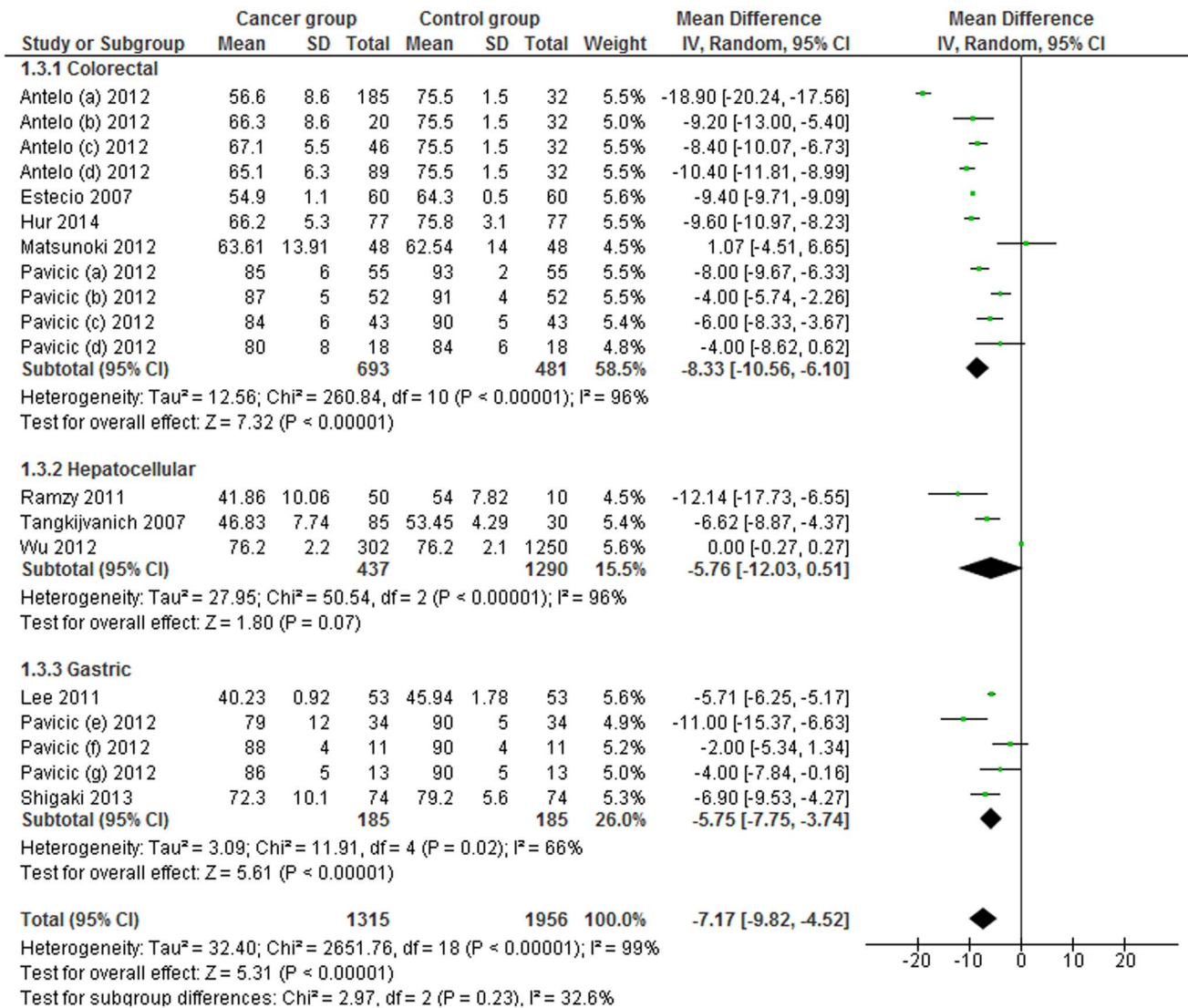
Figure 4. Forest plot of the mean difference of LINE-1 methylation levels between cancer and control groups. Subgroups analysis based on cancer type. doi:10.1371/journal.pone.0109478.g004
