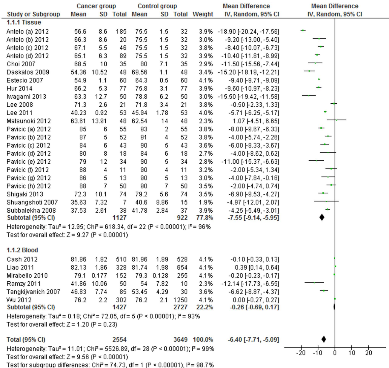
Figure 2. Forest plot of the mean difference of LINE-1 methylation levels between cancer and control groups in tissue and blood samples. Subgroup analysis based on sample type. doi:10.1371/journal.pone.0109478.g002
