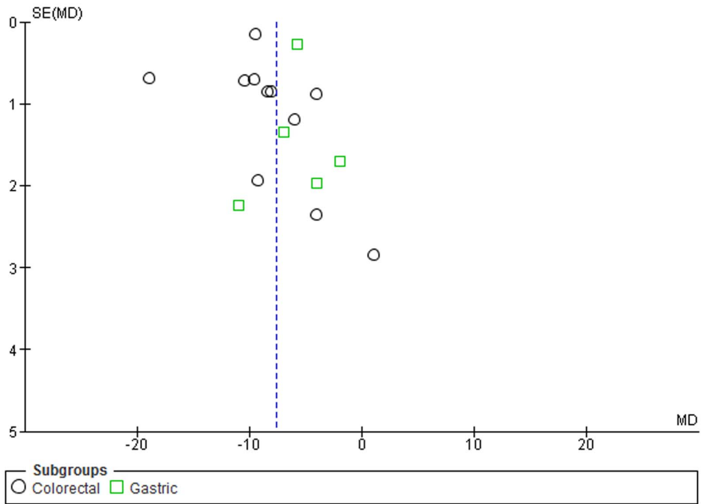
Figure 10. Funnel plot. Subgroup analysis based on cancer type in tissue samples. doi:10.1371/journal.pone.0109478.g010
