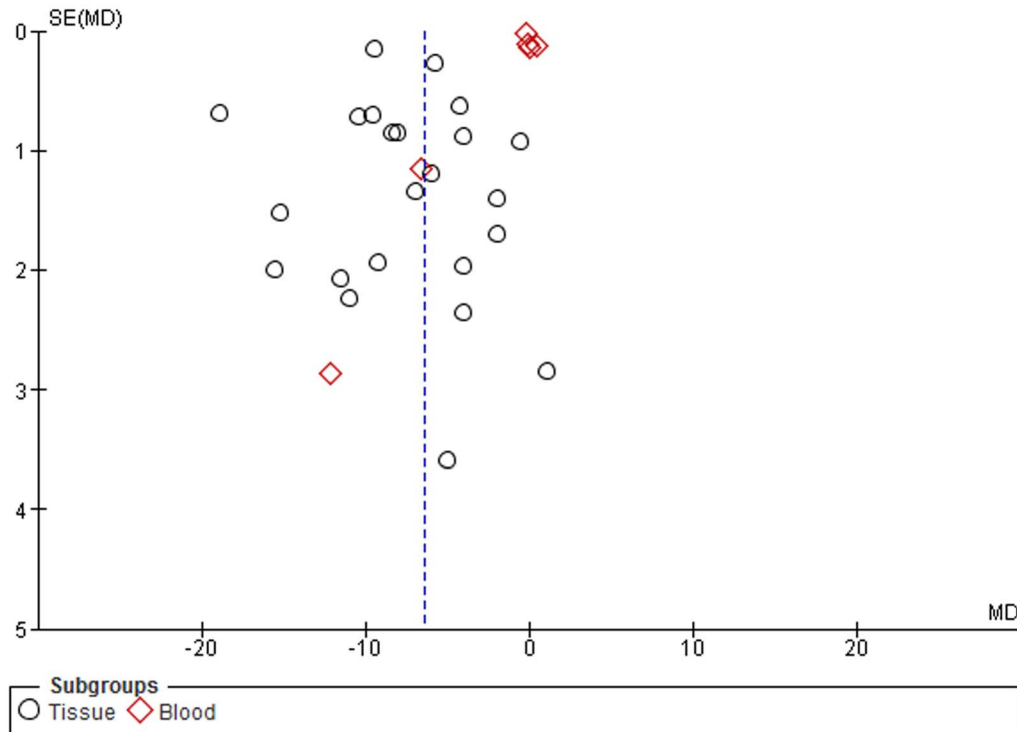
Figure 7. Funnel plot. Subgroup analysis based on sample type. doi:10.1371/journal.pone.0109478.g007
