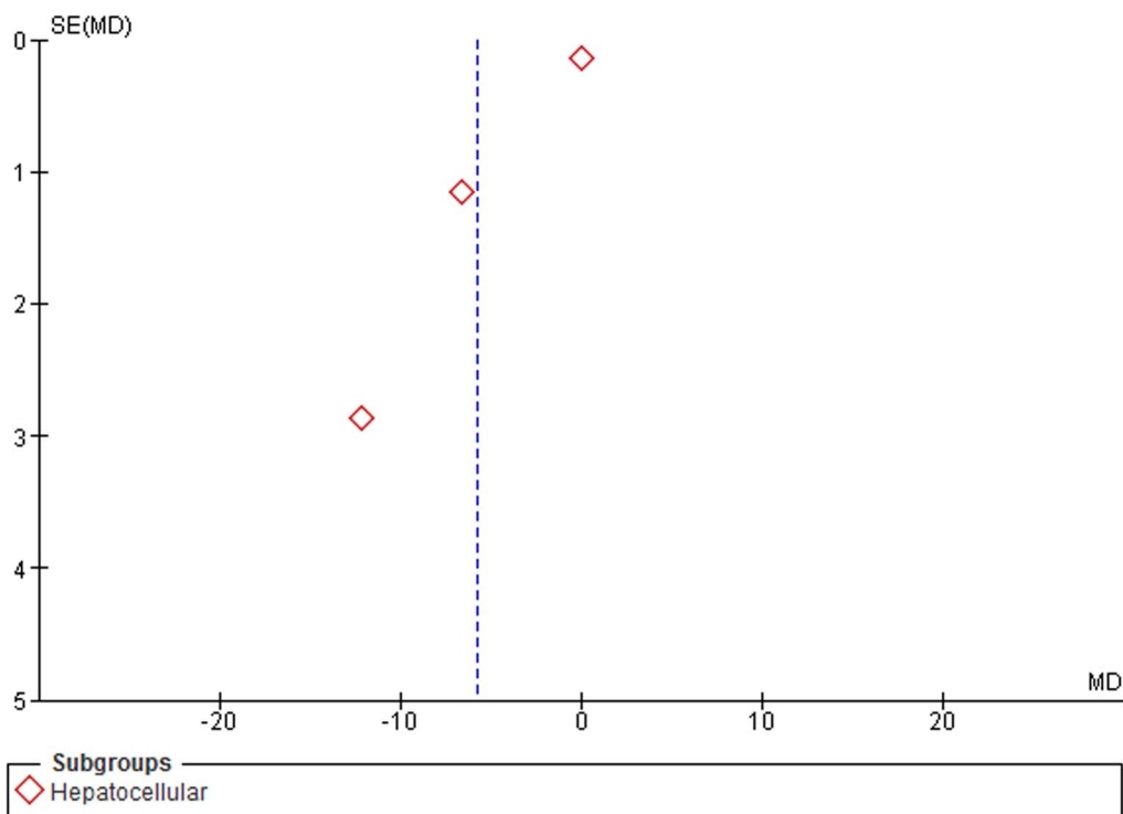
Figure 9. Funnel plot. Subgroup analysis based on cancer type in blood samples. doi:10.1371/journal.pone.0109478.g009
