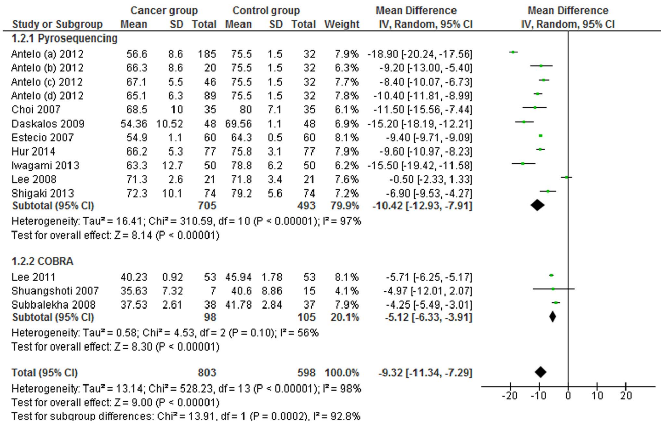
Figure 6. Forest plot of the mean difference of LINE-1 methylation levels between cancer and control groups in tissue samples. Subgroups analysis based on method. doi:10.1371/journal.pone.0109478.g006
