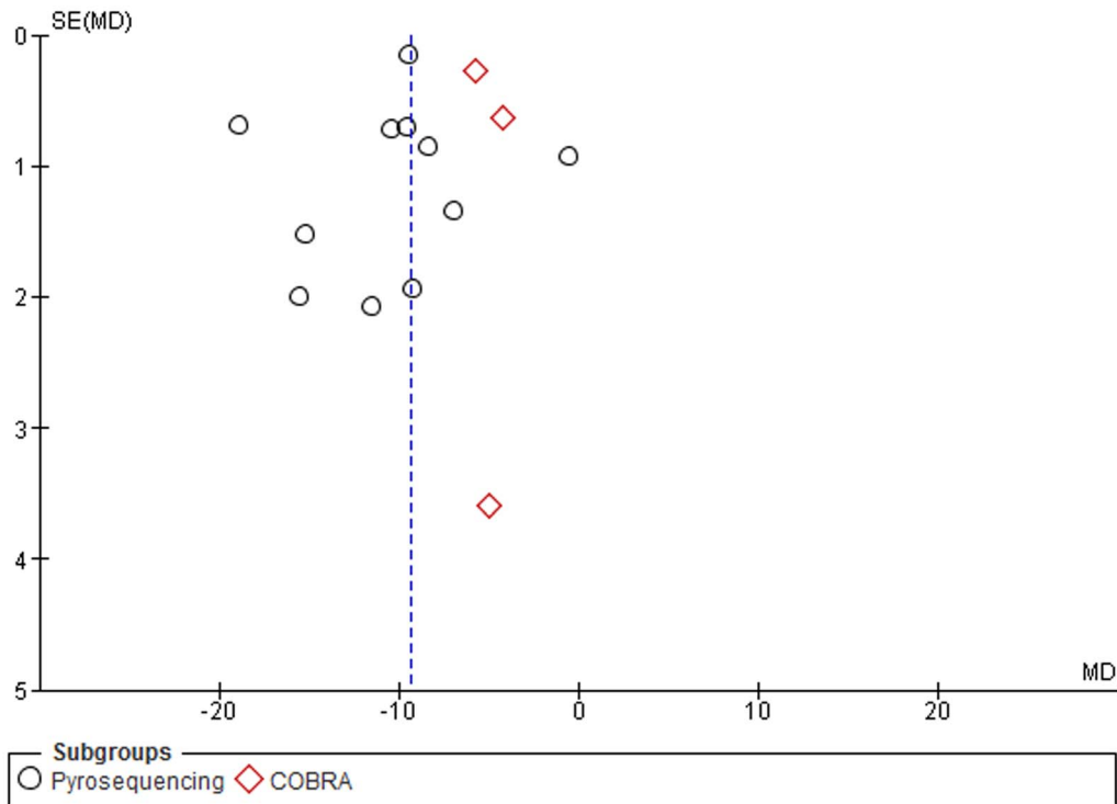
Figure 12. Funnel plot. Subgroup analysis based on detection method in tissue samples. doi:10.1371/journal.pone.0109478.g012
