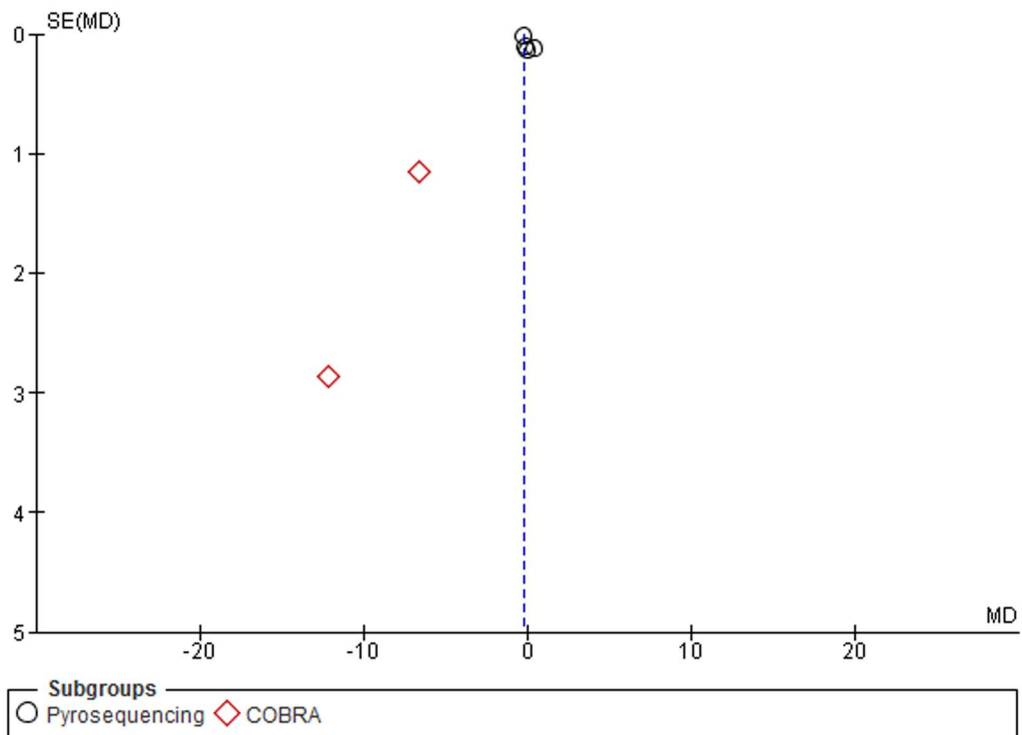
Figure 11. Funnel plot. Subgroup analysis based on detection method in blood samples. doi:10.1371/journal.pone.0109478.g011
