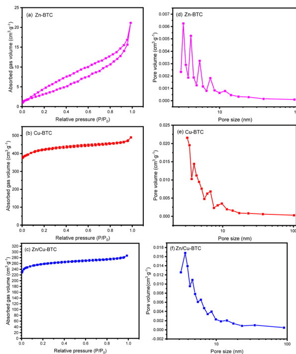
Fig. 3 The \text{N}_2 adsorption–desorption isotherms (a–c) and pore size distribution (d–f) of Zn-BTC, Cu-BTC and Zn/Cu-BTC.
