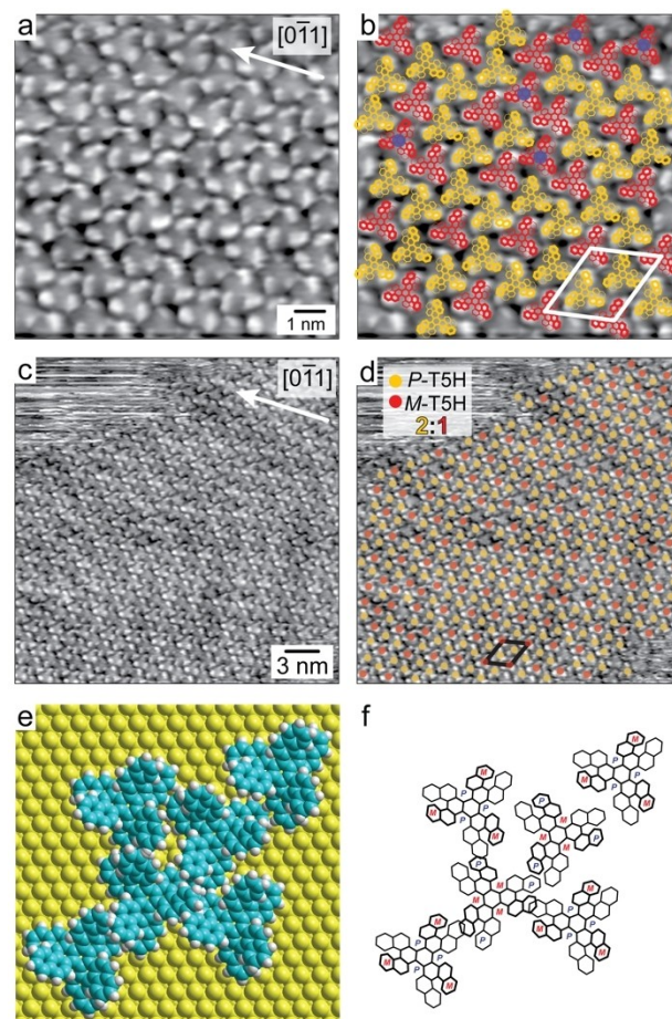
Figure 1. STM images (see Supporting Information for parameters) of self-assembled T[5]H molecules at monolayer coverage on Au(111). (a) High resolution STM image. A white arrow denotes a high symmetry direction of the (111) surface. A single molecule appears as windmill, allowing assignment of absolute configuration. (b) Corresponding STM image with superposition of molecular models (yellow: ( outer-P )-T[5]H, red: ( outer-M )-T5H). The unit cell is indicated by a white rhomb. It contains 2 ( outer-P )-T[5]H and 1 ( outer-M )-T5H. The ( outer-M )-T5H at the corners of the unit cell are separated by 2.36 nm. The blue dots mark deviations from the opposite-handedness-scheme of adjacent molecules. (c, d) Overview STM images including in part annotation with colored dots with same code as in (b). The Au(111) herringbone reconstruction underneath the molecular layer contributes to the STM contrast. (e) Full-space model of molecular arrangement in the unit cell. (f) Adaptation of model shown in (e) with carbon frame only. The molecular unit cell is commensurate to the Au(111) surface (see Supporting Information Figure S1 for more details on the unit cell).
