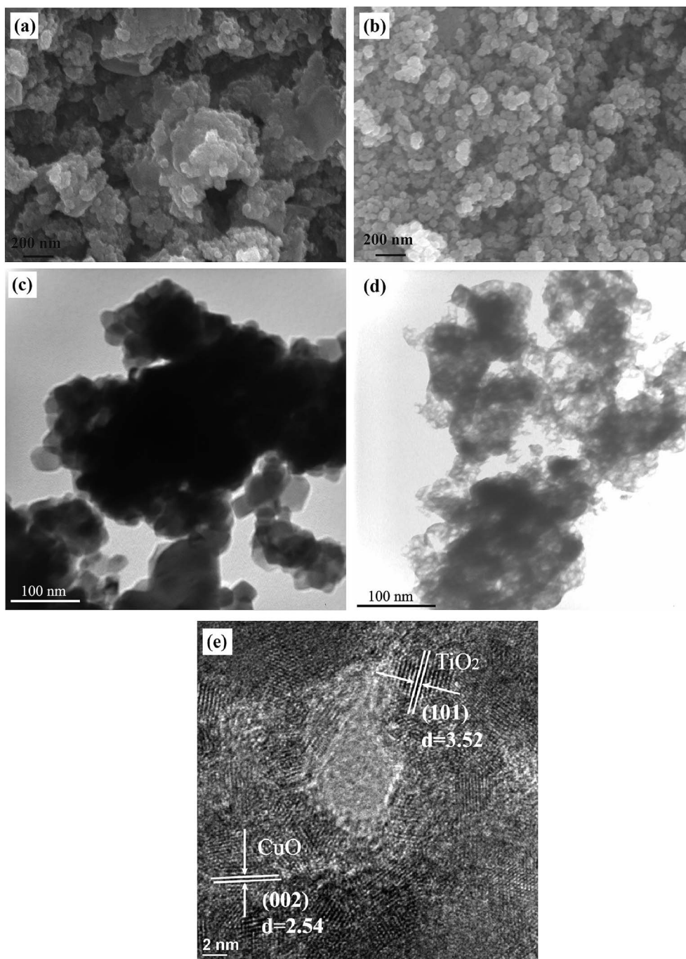
Fig. 4 SEM images of (a) \text{TiO}_2 and (b) \text{CuO/TiO}_2 , TEM images of (c) \text{TiO}_2 and (d) \text{CuO/TiO}_2 , and HR-TEM image (e) of \text{CuO/TiO}_2 catalyst.
