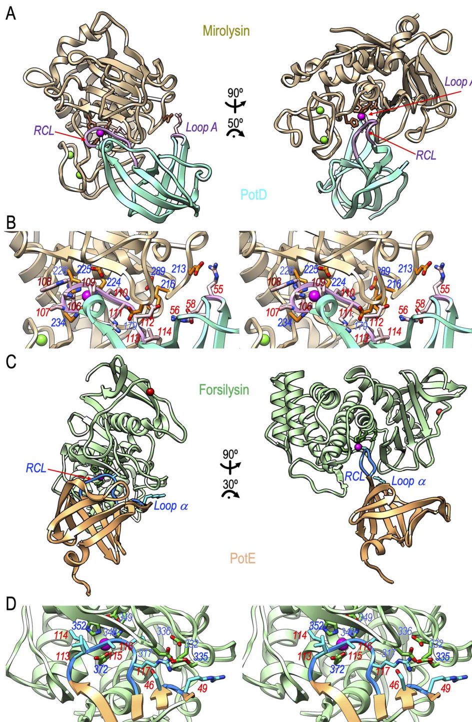
Fig. 8 Models of PotD and PotE complexes with peptidases. (A) Ribbon-plot of PotD (in cyan; RCL and loop A in plum) in the modelled complex with the catalytic domain of miroylysin (in tan) in two orientations (left and right). In the left panel, the peptidase is shown in a similar orientation with respect to its active-site cleft as MMP-12 in Fig. 7A. The catalytic zinc of the peptidase is shown as a magenta sphere coordinated by three histidine residues (H 224 , H 228 and H 234 ; brown sticks). The two calcium cations (green spheres) are also displayed, as are the general base/acid glutamate (E 225 ) and E 213 . The most relevant residue of PotD potentially engaged in inhibition (K 110 ), as well as ancillary R 55 , are further displayed as pink sticks. (B) Close up of a similar view as shown in (A, left) in stereo, focusing on the predicted interaction between PotD and miroylysin in the active-site cleft. Relevant residues of the peptidase and inhibitor are shown as sticks and are numbered in blue and red, respectively. (C) Ribbon-plot of PotE (in orange; RCL and loop \alpha in blue) in the modelled complex with the forsilylin catalytic domain model (in light green) in two orientations (left and right). In the left panel, the peptidase is shown in a similar orientation with respect to its active-site cleft as MMP-12 in Fig. 7A. The catalytic zinc of the peptidase is shown as a magenta sphere coordinated by three residues (H 348 , H 352 and E 372 ; green sticks). A predicted calcium cation (red sphere) is also displayed, as is the general base/acid glutamate (E 349 ). The most relevant residues of PotE potentially engaged in inhibition (I 116 from the RCL and R 49 from loop \alpha ) are displayed as cyan sticks. (D) Close up of a similar view as shown in (A, left) in stereo, focusing on the predicted interaction between PotE and forsilylin in the active-site cleft. Relevant residues of the peptidase and inhibitor are shown as sticks and are numbered in blue and red, respectively.
