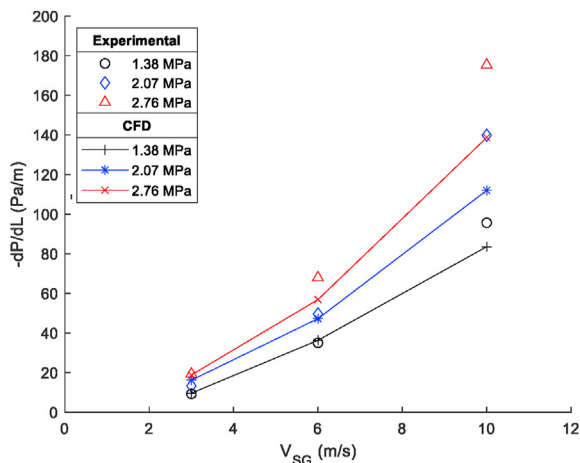
Figure 14. Effect of operating pressure and gas velocities ( V_{SG} ) on experimental and CFD pressure drop ( -dP/dL ).
