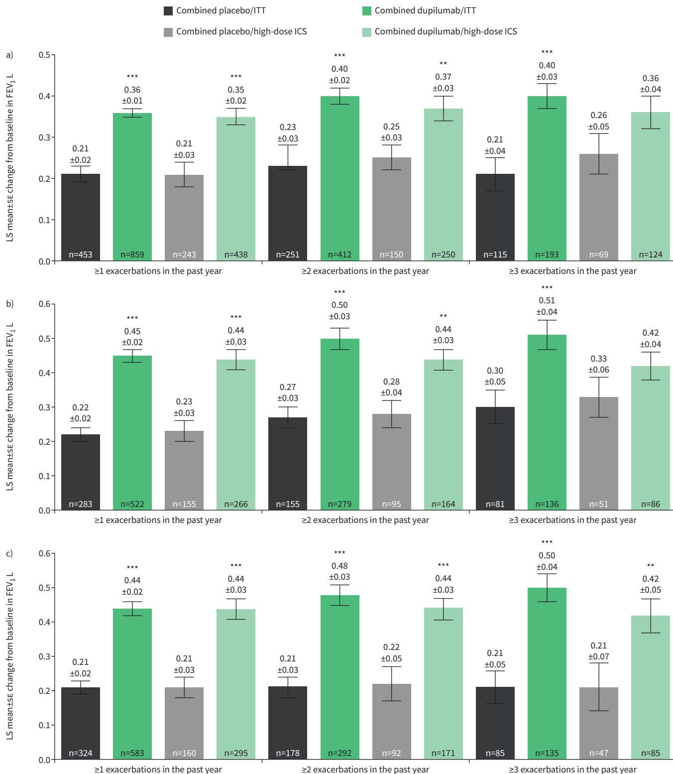
FIGURE 2 Least squares (LS) mean±SE change from baseline at week 12 in pre-bronchodilator forced expiratory volume in 1 s (FEV 1 ) in patients categorised by a) baseline blood eosinophils \geq 150 \text{ cells}\cdot\mu\text{L}^{-1} , b) baseline blood eosinophils \geq 300 \text{ cells}\cdot\mu\text{L}^{-1} and c) baseline exhaled nitric oxide fraction \geq 25 \text{ ppb} (intention-to-treat (ITT) or high-dose inhaled corticosteroid (ICS)). **: p < 0.01 ; ***: p < 0.001 versus placebo.
