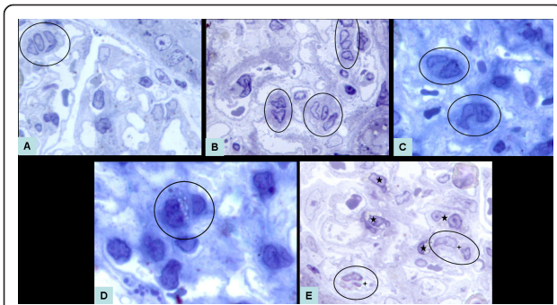
Figure 1 Expression of PDEC GF in the control and experimental groups. Control group has no immunopositivity (A). Pre-proteinuria group has weak immunopositivity around the mesangial matrix (B). Acute group has moderate immunopositivity around the mesangial matrix regions (C). Chronic group has very strong immunopositivity in the cells of mesangial matrix regions (D). PDEC GF- Negative chronic control group has no positivity (E) X40. Positive control is malignant melanoma tissue and has strong immunopositivity in stromal cells (F) X20.
