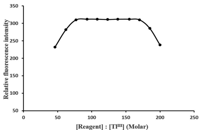
Fig. 6 Effect of the reagent (PQCTA : Tl III molar concentration, i.e. , molar ratio of PQCTA/Tl III ) on the fluorescence of the Tl III -PQCTA system.
