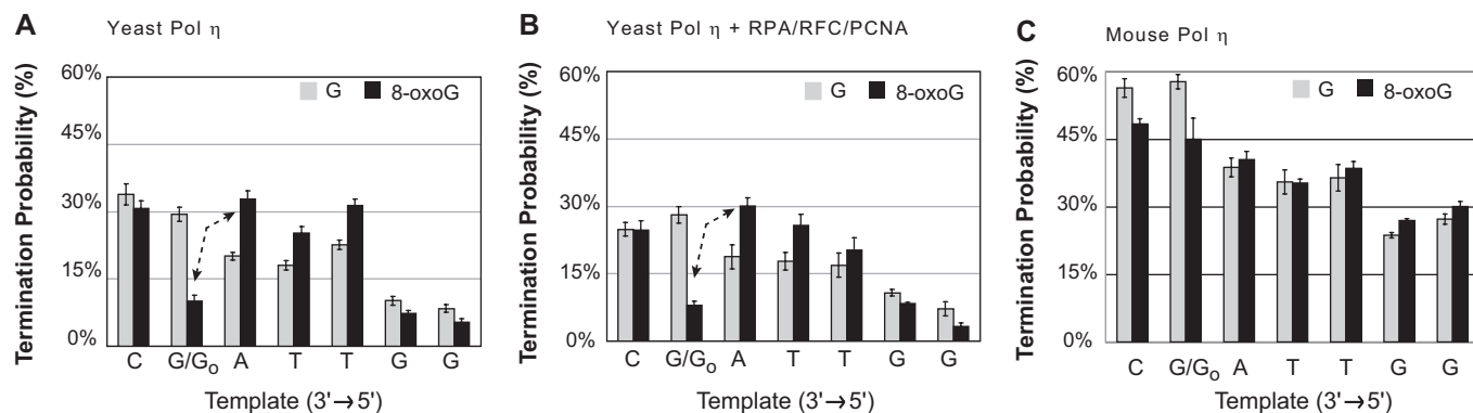
Figure 4. Termination probability analysis during 8-oxoG bypass by Pol \eta . Gel images of reaction products seen in Figure 3 were quantified using ImageQuant software, as described previously (39,41). (A) Graph of termination probability (vertical axis, 0–60%) at each of the first seven incorporations (horizontal axis) for S. cerevisiae Pol \eta without accessory proteins. Undamaged template and 8-oxoG template values are indicated by light gray and black bars, respectively. Error bars are the standard deviation for six measurements (three time points each for two separate experiments). The switch from low to high termination probability after 8-oxoG has been bypassed is indicated with dashed-line arrows. (B) Graph of termination probability for S. cerevisiae Pol \eta with RPA, RFC and PCNA. Details are the same as in (A). (C) Graph of termination probability for mouse Pol \eta without accessory proteins on a 45-mer template (see ‘Materials and methods’ section). Note that mouse and human Pol \eta display nearly identical properties (41,49,51).
