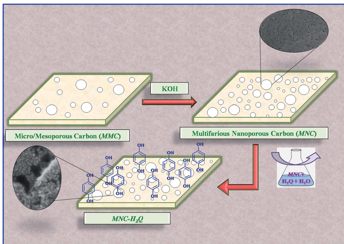
Fig. 1 Schematic representation of the preparation of MNC from micro/mesoporous carbon (MMC) and subsequent formation of MNC- \text{H}_2\text{Q} from MNC.
