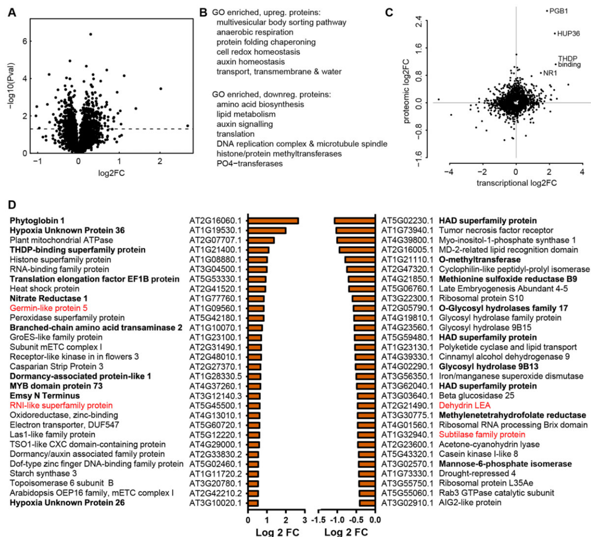
Figure 3 Ethylene treatment modulates the Arabidopsis root tip proteome. A, Volcano plots showing the quantitative change in protein abundance upon 4 h of ethylene treatment (5 \mu\text{L}\cdot\text{L}^{-1} ; the pretreatment) and the statistical significance. Dashed line indicates P = 0.05 . B, Key processes, functions and locations enriched among up and down regulated proteins based on gene ontology (GO) enrichment. Full lists of GO terms are available in the Supplemental Data (Sheet 10) . C, Direct comparison of transcriptomic and proteomic response for individual genes. D, The 30 strongest up and down regulated proteins are shown based on fold change. Proteins in bold are also regulated in the corresponding direction at the transcript level. Proteins in red showed an opposite response at the transcript level. All proteins shown are significantly different ( P < 0.05 , Student's t test, n = 5 ).
