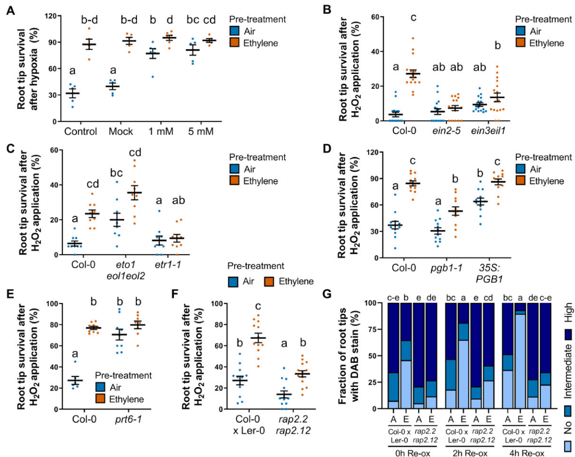
Figure 5 Ethylene improves oxidative stress survival. A, Root tip survival of 4-day-old Arabidopsis (Col-0) seedlings after 4 h of air or \sim 5 \mu\text{L}\cdot\text{L}^{-1} ethylene treatment in combination with application of mock or 1-mM or 5-mM ROS scavenger KI, followed by 4 h of hypoxia and 3 days of recovery ( n = 5 plates containing approximately 46 seedlings). B–F, Root tip survival of (B) Col-0 and ethylene insensitive mutants ein2-5 and ein3eil1 , (C) Col-0, ethylene enhanced biosynthesis mutant eto1eol1eol2 and receptor mutant etr1-1 , (D) Col-0, pgb1-1 and 35S:PGB1, (E) Col-0, N-degron mutant prt6-1 (Col-0 background) and a (F) Col-0 x Ler-0 cross and ERFVII double mutant rap2.2rap2.12 (Col-0 x Ler-0 background) after 4 h of air or \sim 5 \mu\text{L}\cdot\text{L}^{-1} ethylene treatment followed by application of 5 \mu\text{L} of H_2O_2 (6 mM) on each single root tip and 3 days of recovery. Statistically similar groups are indicated using the same letter ( n = 5 –16 rows containing approximately 23 seedlings). G, Proportion of WT (Col-0 x Ler-0 background) or ERFVII double mutant rap2.2rap2.12 (Col-0 x Ler-0 background) root tips showing H_2O_2 (DAB) staining after air or \sim 5 \mu\text{L}\cdot\text{L}^{-1} ethylene treatment followed by 4 h of hypoxia and 2 h of re-oxygenation. Statistically similar groups are indicated per timepoint using the same letter ( n = 146 –180 root tips). Dots indicate a single row/plate of seedlings, error bars represent SEM (A–F). For (A–G) the letters indicate significantly indistinguishable groups ( P < 0.05 ) based on Tukey's [AQ]HSD following a generalized linear model with binomial link function (GLM-binomial). The effect of ethylene on ROS tolerance or DAB staining was tested for with an interaction term in a GLM-binomial with a genotype (WT and mutant) and pretreatment (ethylene-control) effect. Interaction terms for H_2O_2 tolerance were statistically significant for ein2-5 ( P = 2\text{e-}4 ), ein3eil1 ( P = 1\text{e-}5 ), etr1-1 ( P = 0.04 ), pgb1 ( P = 1\text{e-}4 ), 35S:PGB1 ( P = 0.002 ), prt6-1 ( P = 3\text{e-}8 ), but not for eto1eol1eol2 ( P = 0.1541 ), and rap2.12/2.2 ( P = 0.21 ). DAB staining interaction terms were 0 h ( P = 0.01 ), 2 h ( P = 0.04 ), 4 h ( P = 9\text{e-}6 ).
