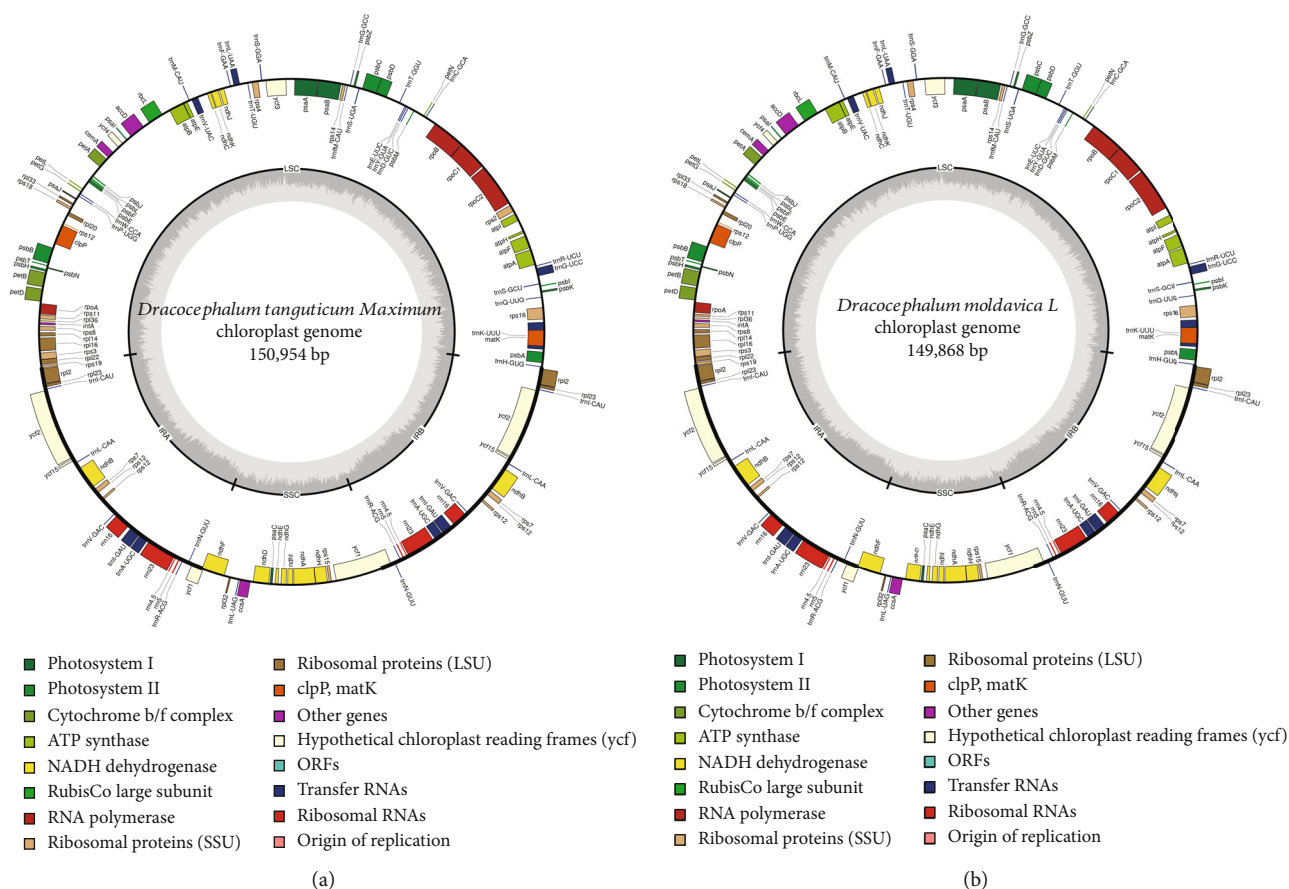
FIGURE 1: (a) D. tanguticum chloroplast genome. (b) D. moldavica chloroplast genome. The genes that code forward are on the outside of the circle, and the genes that code backward are on the inside. The legend identifies genes with different functions.
