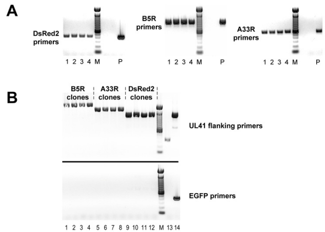
Figure 7 PCR Analysis of HSV-2 BAC recombinants. (A) Insert-specific PCR of 4 individual clones each of HSV2-BAC recombinants containing an inserted DsRed2 (left panel), vaccinia virus B5R (middle panel) or vaccinia virus A33R gene (right panel). Lane M - 100 bp molecular size markers. Lane P - Specific plasmid controls containing the genes for DsRed2 , B5R , A33R , respectively (from left to right). Sizes of PCR products are: DsRed2 - 424 bp; B5R - 1014 bp; A33R - 586 bp. (B) UL41 and EGFP PCR analysis of 4 individual clones each of HSV2-BAC recombinants containing an inserted vaccinia virus B5R (lanes 1-4), vaccinia virus A33R gene (lanes 5-7), or DsRed2 gene (lanes 9-12). Lane M - 100 bp molecular size markers. Lane 13 - HSV2-BAC. Lane 14 - DEST-BAC. The top half of the gel shows the PCR products generated with UL41 primers for each clone. Sizes of UL41 PCR products are: B5R - 2280 bp; A33R - 1850 bp; DsRed2 - 1290 bp ( DsRed2 ); HSV2-BAC - 342 bp; UL41 PCR of DEST-BAC - 1320 bp). The bottom half of the gel shows the PCR products using EGFP primers for each clone, confirming the absence of the EGFP in each recombinant. Size of EGFP PCR product of DEST-BAC is 433 bp (lane 14).
