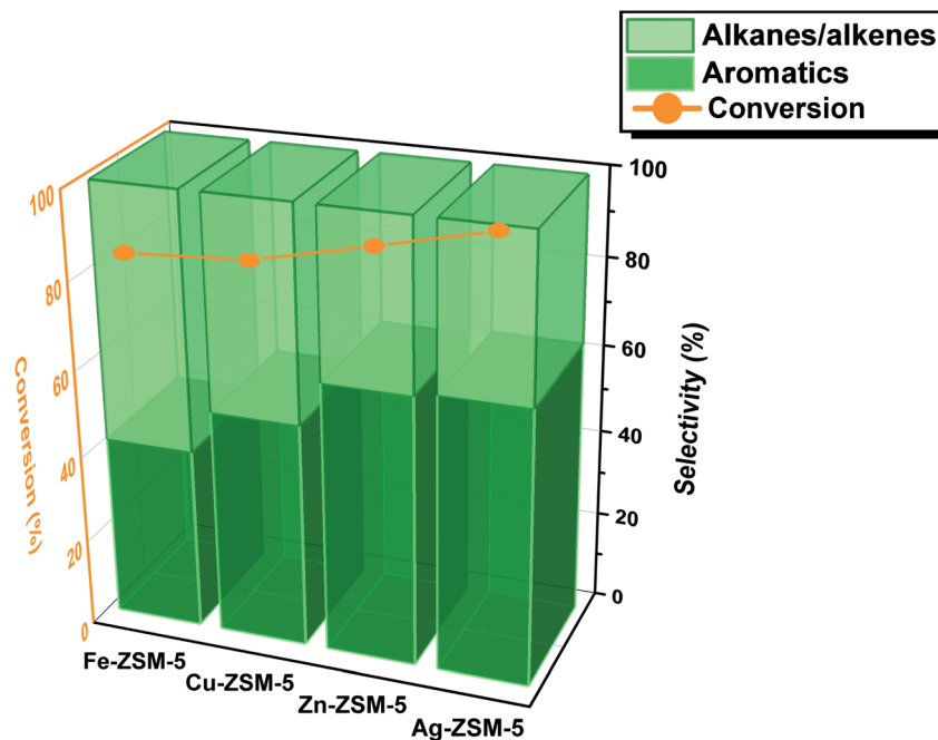
Fig. 1 MTA catalytic results for H-ZSM-5 exchanged with metal ions including Fe, Cu, Zn and Ag. Liquid methanol with a flow rate of 0.016 mL min -1 was pumped into a fixed bed stainless steel reactor that hosted 0.5 g of the ion-exchanged catalysts sandwiched by quartz wool plugs. The carrier gas was N 2 with a feed rate of 3 mL min -1 at reaction conditions of 397 °C and 10 bar. The conversion and selectivity are taken at steady-state, and the total selectivity with respect to converted methanol to all these products is 100%; measurement errors by gas chromatography are within 10%.
