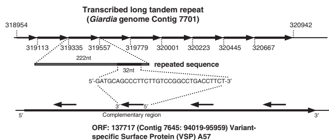
Figure 3. Tandem repeats of the Girep-1 RNA. Each fragment coloured in grey represents a repeating unit (222 nt in length, with the first unit lacking the 5' 63 nt and the last unit extending 54 nt at 3' end) on Girep-1 RNA. Each 32 nt fragment coloured in black represents the repeating Girep-1 sequence that is complementary to the various-surface-protein (VSP) gene.
