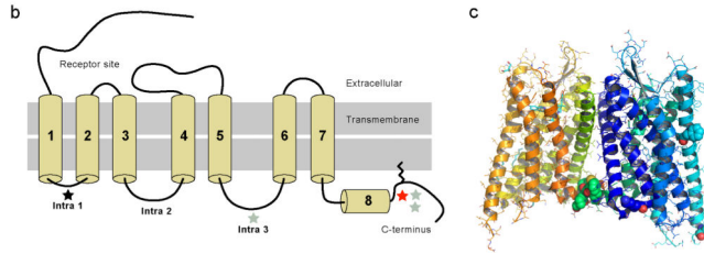
Extended Data Figure 2. Rapid Evolution of EDNRB1 a , Alignments of EDNRB1 in cichlids with human (HS), zebrafish (DAR) and medaka (ORL). Black star denotes site shown to be required to activate SRF in human by interacting with the G protein G13 (ref. 40). Red star denotes site that may affect the anchoring of the C terminus of EDNRB1 to the transmembrane domain 41 . Highlighted are amino acid substitution in the ancestor of haplochromine and lamprologini (blue) and in the ancestor of haplochromine (red). b , Location of substitutions on 7 transmembrane domain representation (Adapted from ref. 42 Science 318, 1453–1455. Reprinted with permission from AAAS.). c , Sites (spheres) on the structure of the human kappa opioid receptor in complex (4DJH). Only the right homodimer is annotated.
