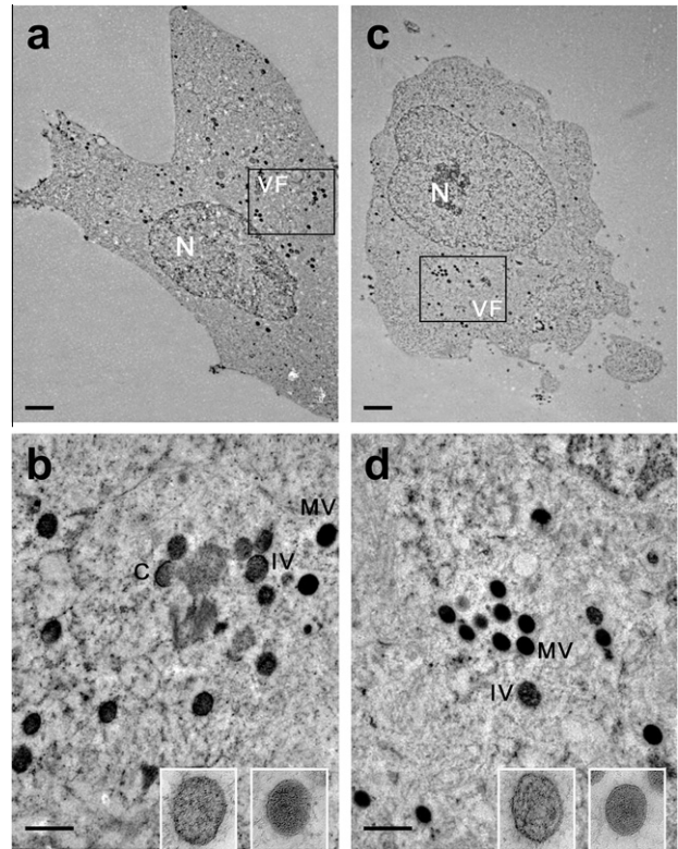
Fig. 7. Ultrastructure comparison after X-ray irradiation. HZB2 grids used for cryo X-ray tomography were subjected to freeze-substitution and embedding in Lowicryl resin. Areas containing irradiated and non-irradiated cells were identified based on grid marks and features. Thin sections were obtained by ultramicrotomy and observed by electron microscopy. (a) Cell section from a non-irradiated area. N marks the position of the nucleus, VF marks a viral factory. Scale bar represents 2 microns. (b) Higher magnification detail of the cytoplasm from (a). C shows a viral crescent, IV immature virus and MV mature virus. The left inset shows a magnified view of an IV, and the right inset a MV. Scale bar represents 500 nm. (c) Section of a heavily X-ray irradiated cell used to collect two full X-ray tomographic data sets. N marks the position of the nucleus, VF marks a viral factory. The scale is the same as in (a). (d) Higher magnification detail of the cytoplasm from (c). IV shows immature virus and MV mature virus. The left inset shows a magnified view of an IV, and the right inset a MV. Scale bar represents 500 nm.
