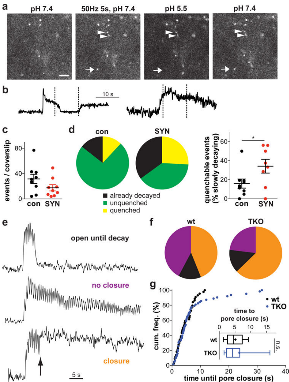
Figure 3. \alpha -Synuclein influences fusion pore closure in neurons (a) Rodent hippocampal neurons were transfected with BDNF-pHluorin and imaged 14–20 days later, stimulating at 50 Hz for 5 s followed immediately by quenching of the cell surface fluorescence at pH 5.5. The arrow indicates an event quenchable at low pH, and the arrowheads events resistant to quenching. Scale bar, 5 \mu m. (b) Sample BDNF-pHluorin traces show sensitivity to quenching by pH 5.5 applied between the dashed lines (left) and resistance to quenching (right). (c) Average event frequency per coverslip (mean \pm SEM) for BDNF-pHluorin expressing rat hippocampal neurons co-transfected with \alpha -synuclein (SYN) or empty vector (con) and stimulated as in (a) (above) ( p = 0.13 by unpaired, two-tailed t test; t(16) = 1.582 ). n = 9 cells from 2 independent cultures (d) Classifying events as
