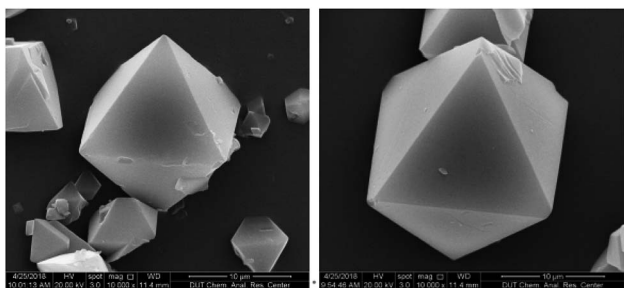
Fig. 2 SEM images of HKUST-1 (left) and Cu/Co-BTC-174 (right).
