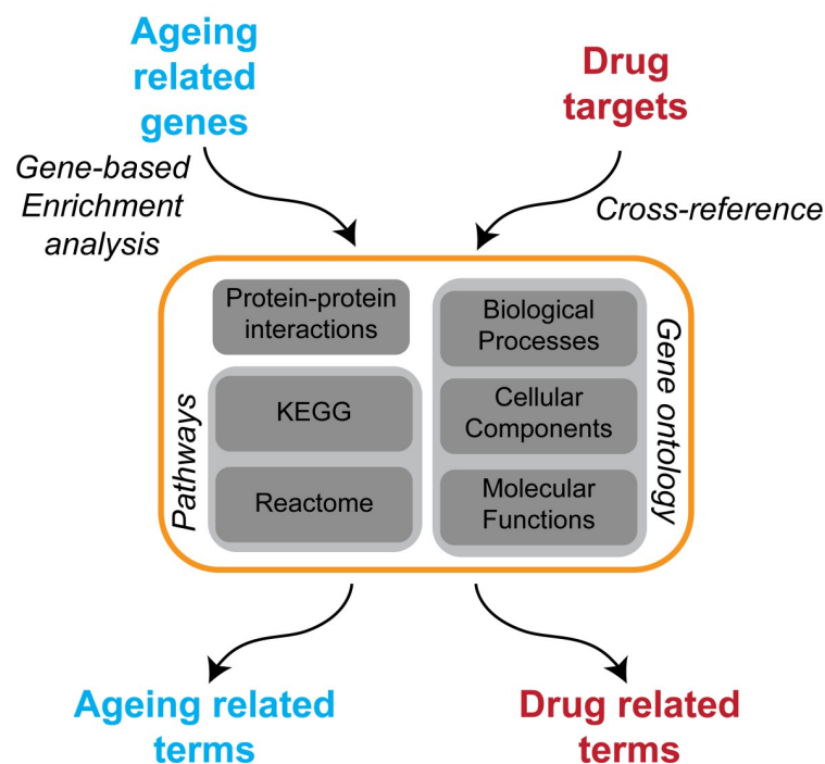
Fig 1. Overview of the methods used in this study to prioritise compounds likely to ameliorate ageing in humans. A) STITCH chemicals were mapped into DrugBank drugs using the UniChem resource programmatically. B) The significance of the drug-ageing inference was calculated using a Fisher's exact test, which calculates the probability that the overlap between two samples (ageing-related genes and drug targets) drawn from the same universe is due to chance. This comparison was made at different biological levels. C) Diagram of the procedure to expand the “gene” information into multiple biological levels. Ageing-related genes were mapped to other levels using an enrichment analysis, while the drugs’ targets were cross-referenced with the list of genes defining each annotation.
