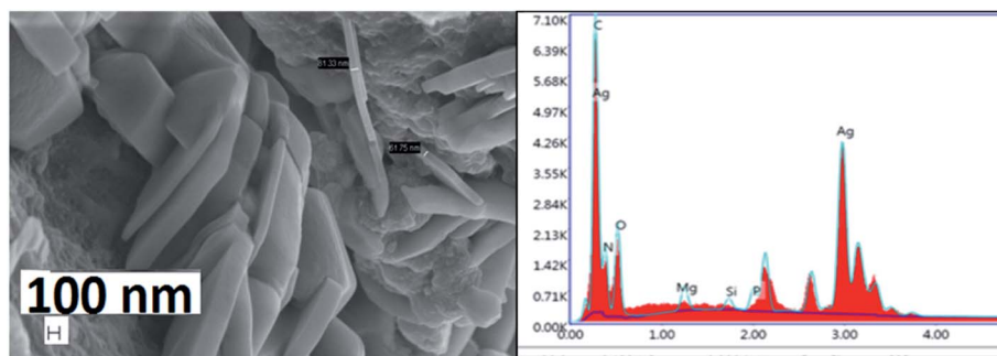
Fig. 11 FESEM/EDX report of freshly synthesized silver nanoplates using Colocasia esculenta leaf extract.
