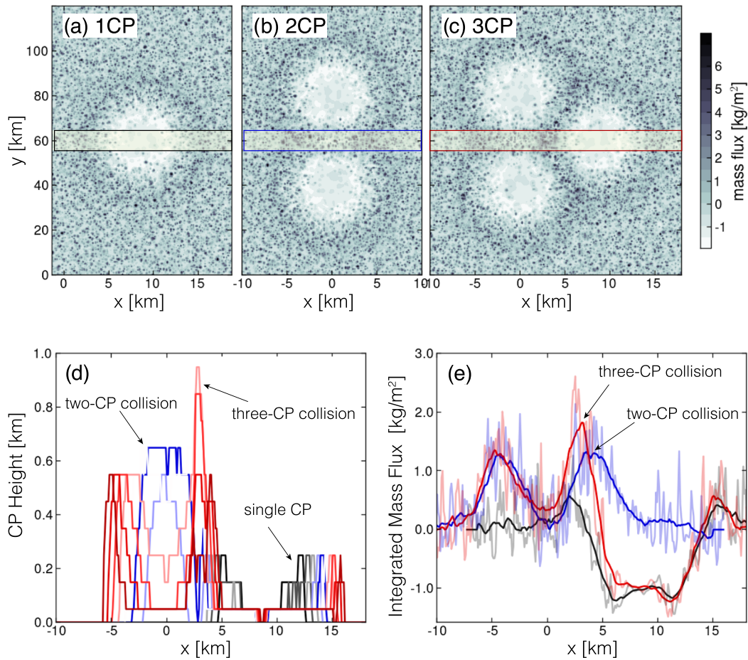
Figure 8. Cold pool height and accumulated vertical mass flux (MF). (a) Horizontal cross section of the accumulated vertical mass flux at z = 1 km for 1CP , integrated from t = 10 min after initialization to t_{3CP} + 10 min. The yellow box indicates the band of width 2 km along which MF is averaged in (e); (b and c) as in (a), but for the 2CP and 3CP simulations ( d = 10 km). The same integration time window is used for each simulation, to ensure meaningful comparison. (d) Cross sections of the CP height in 3CP along the box indicated in (c) at subsequent time instances (every 100 s from 800–1,600 s): during the single CP phase (gray to black), two-CP phase ( t_0 \leq t < t_{2CP} ; light to dark blue), and three-CP phase ( t_{2CP} \leq t < t_{3CP} ; light to dark red). (e) Accumulated mass flux at z = 1 km, spatially averaged over a band of 2 km width along the CP collision line, as indicated by the yellow shaded box in (a)–(c) from 1CP simulation (black), 2CP simulation (blue), and 3CP simulation (red).
