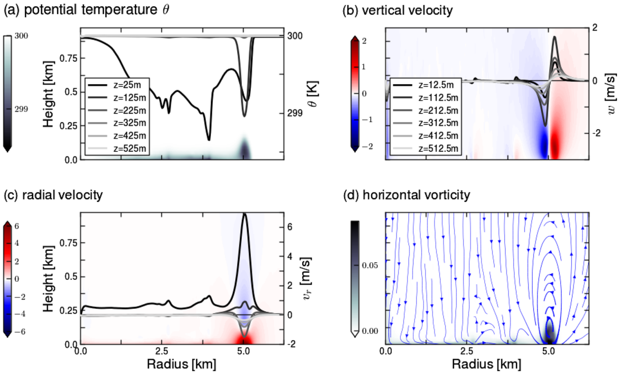
Figure 3. Thermodynamic and dynamic signature of a spreading cold pool. (a) z - r contour plot and cross sections of azimuthally averaged potential temperature \theta , where the cross sections show increasing levels of z (see legend) 20 min after CP initialization (LES parameters analogous to Figure 2). (b) Analogous to (a), but for vertical velocity w ; (c) analogous to (a), but for radial velocity v_r ; (d) similar, but showing vorticity projected onto the radial vector (units of s^{-1} , with superimposed streamlines of v_r and w ).
