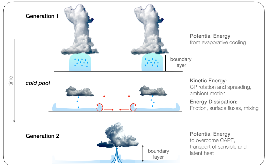
Figure 1. Simplified schematic of CPs linking convective events over space and time by converting the initial potential energy from evaporatively cooled air into kinetic energy of a CP, which by triggering convection transfers it back to potential energy of a second generation event.
