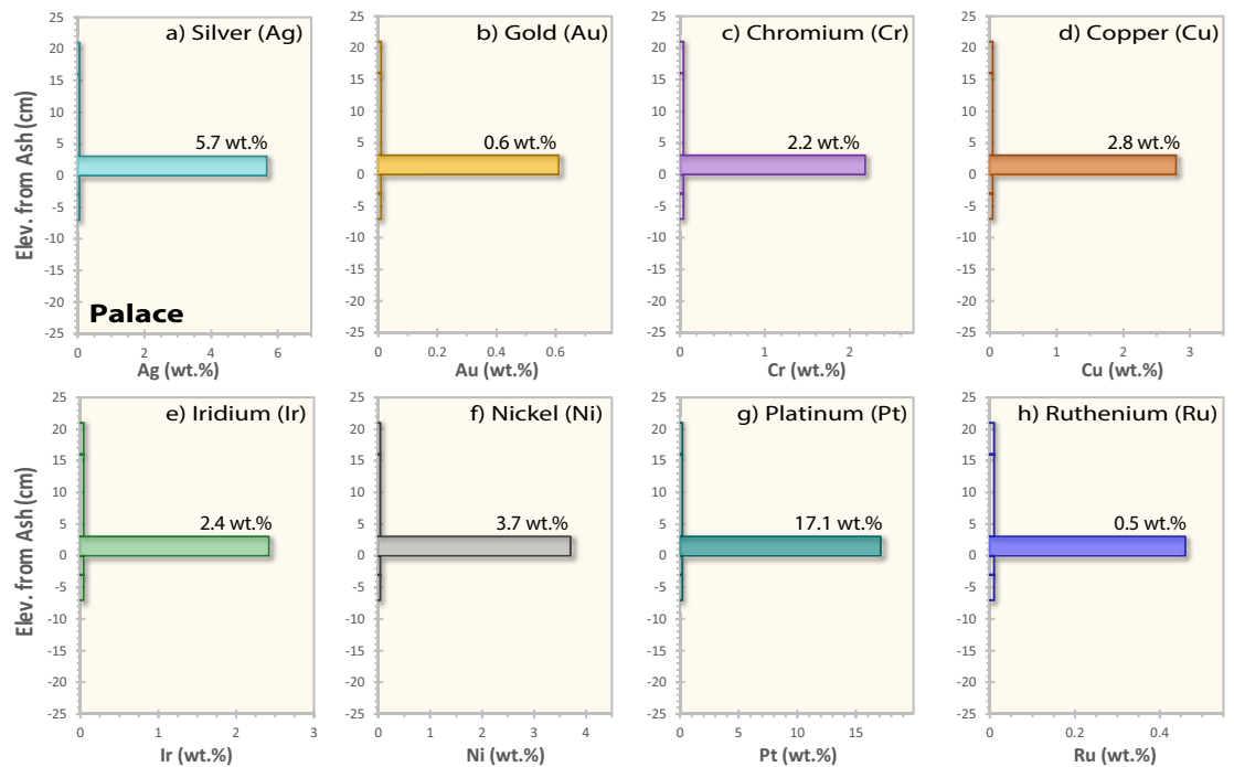
Figure 35. Average composition of selected metal-rich nuggets from the palace. (a–h) Silver (Ag), gold (Au), chromium (Cr), copper (Cu), iridium (Ir), nickel (Ni), platinum (Pt), and ruthenium (Ru), showing wt.% in selected nuggets from the destruction layer of the palace (7GG).
