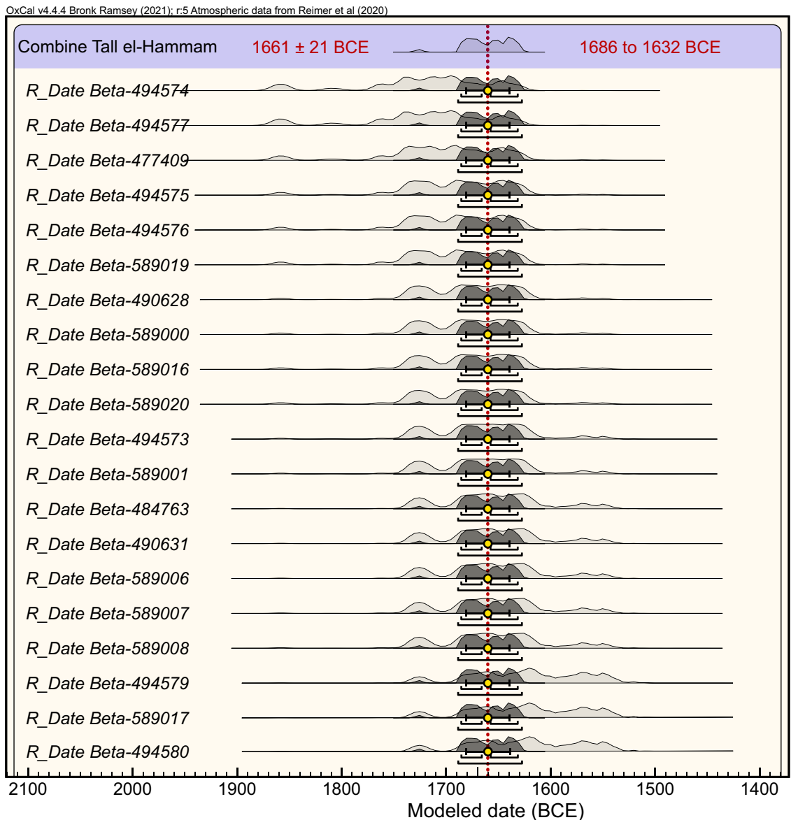
Figure 5. Bayesian analysis. Using OxCal v.4.4.4 18–20 , the ‘Combine’ computer routine determined that 20 of 26 14 C dates are statistically synchronous and likely represent a single event at 1661 \pm 21 BCE (1686–1632 BCE), rounded to 1650 BCE. Light gray curves represent unmodeled calibrated ages; dark gray represents modeled calibrated ages. The white dot beneath the curves equals the mean age, also represented by the red dotted vertical line. Progressively longer brackets beneath curves represent 68% and 94% confidence intervals. The program performed two statistical probability tests to test the robustness of the model. Both the A_{\text{comb}} and Chi Sq statistical tests show a high probability, indicating that the modeled age of 1661 \pm 21 BCE is likely to be accurate.
