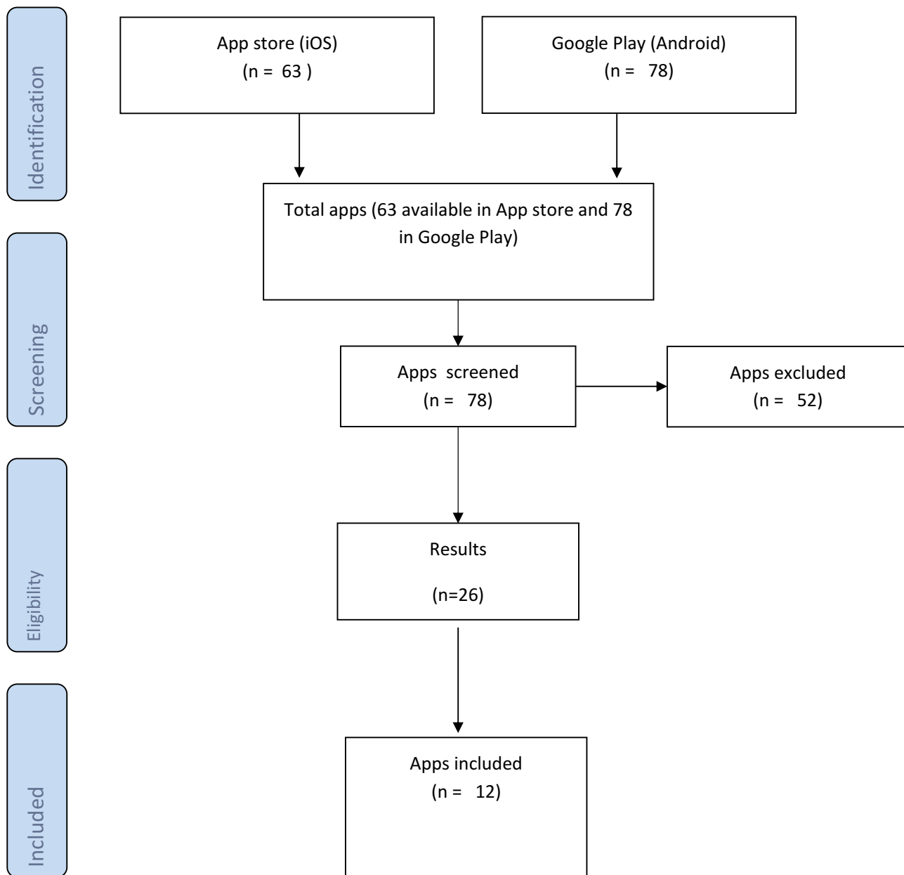
Figure 1 PRISMA flowchart of the search process.
