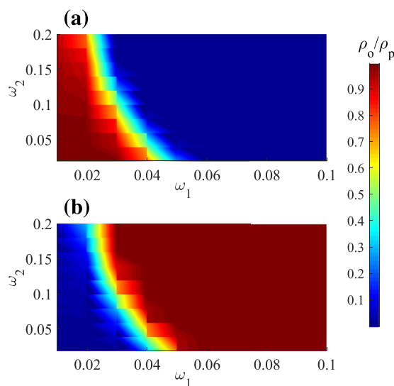
Figure 2. The evolution of (a) the obese density \rho_o and (b) the physical active density \rho_p in the parameter space \omega_1 - \omega_2 . The value of fading coefficient of information spread \eta is 0.2 and the network rewiring probability p_r is 0.5. We delete the extreme values: \omega_1 = 0 and \omega_2 = 0 .
