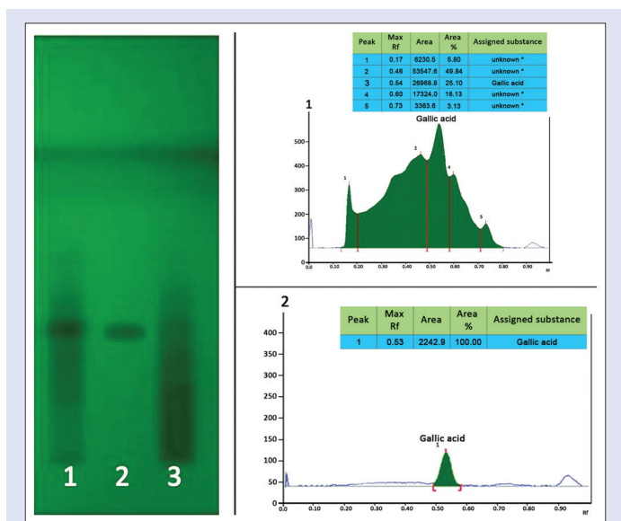
Figure 2: High-performance thin layer chromatography fingerprinting profile identifying the presence of gallic acid in Sansevieria roxburghiana ethyl acetate fraction. Track 1-ethyl acetate fraction of Sansevieria roxburghiana 5 µl; Track 2-gallic acid; Track 3-SREA 10 µl
